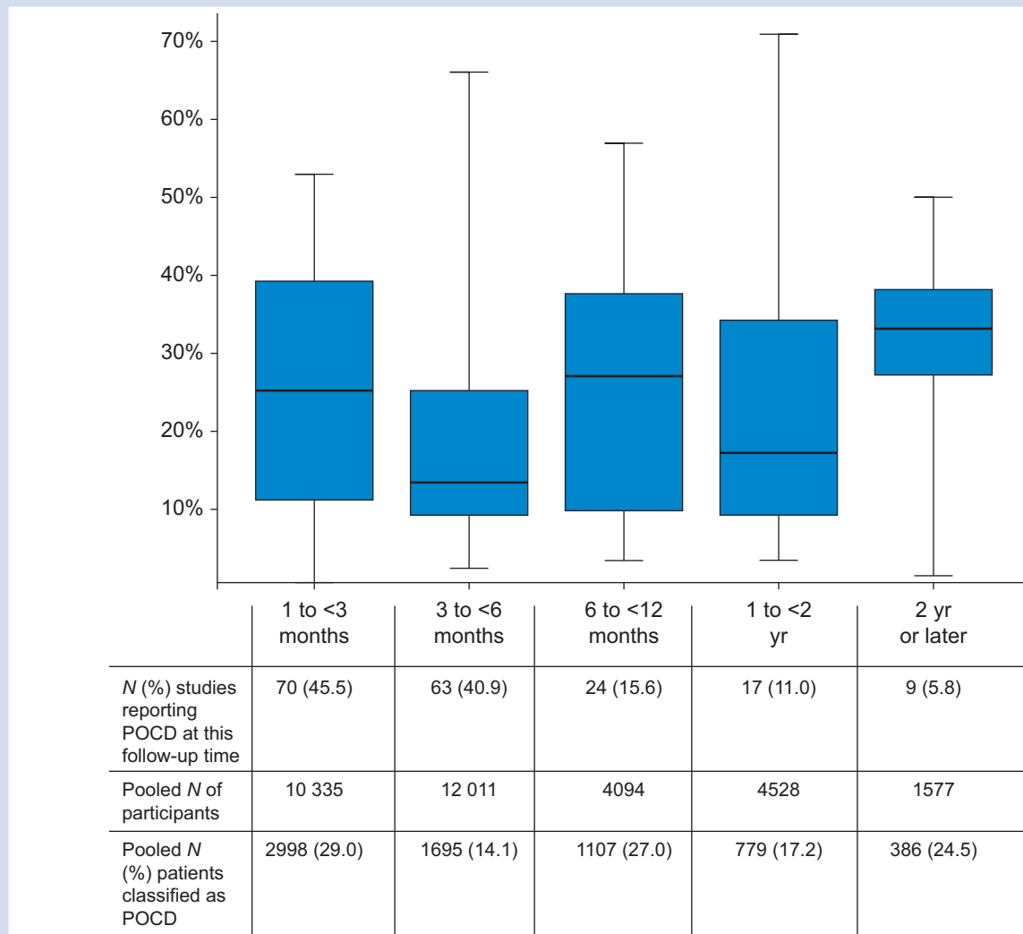
Fig 3. Pooled analysis of studies reporting postoperative cognitive dysfunction (POCD) as a dichotomous outcome and with available data at least one follow-up time after 1 month ( n=154 ). Box plot represents median reported POCD incidence, 25th and 75th percentile, whiskers represent 1.5*inter-quartile range below 25th and above 75th percentile.
