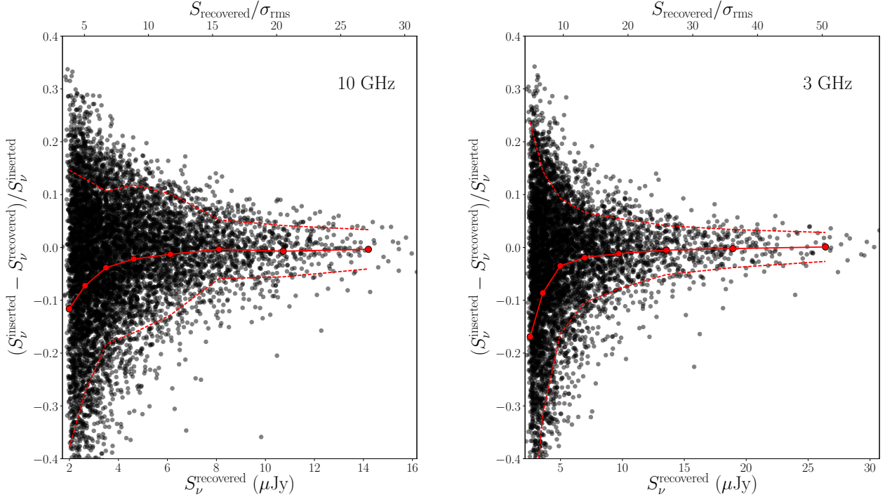
Figure 7. The simulated ratio of (inserted flux density - recovered flux density) to inserted flux density as a function of the recovered flux density. The left panel shows the distribution for the 10 GHz image and the right panel shows the distribution for the 3 GHz image. The solid red line denotes the median of 8 logarithmic bins (indicated by the red points) across the flux density range and the dashed lines mark the 1\sigma upper and lower bounds in those bins. The effect of flux boosting at the faint end is illustrated by the rapid downturn below about 3\mu\text{Jy} for 10 GHz and 3 GHz.
