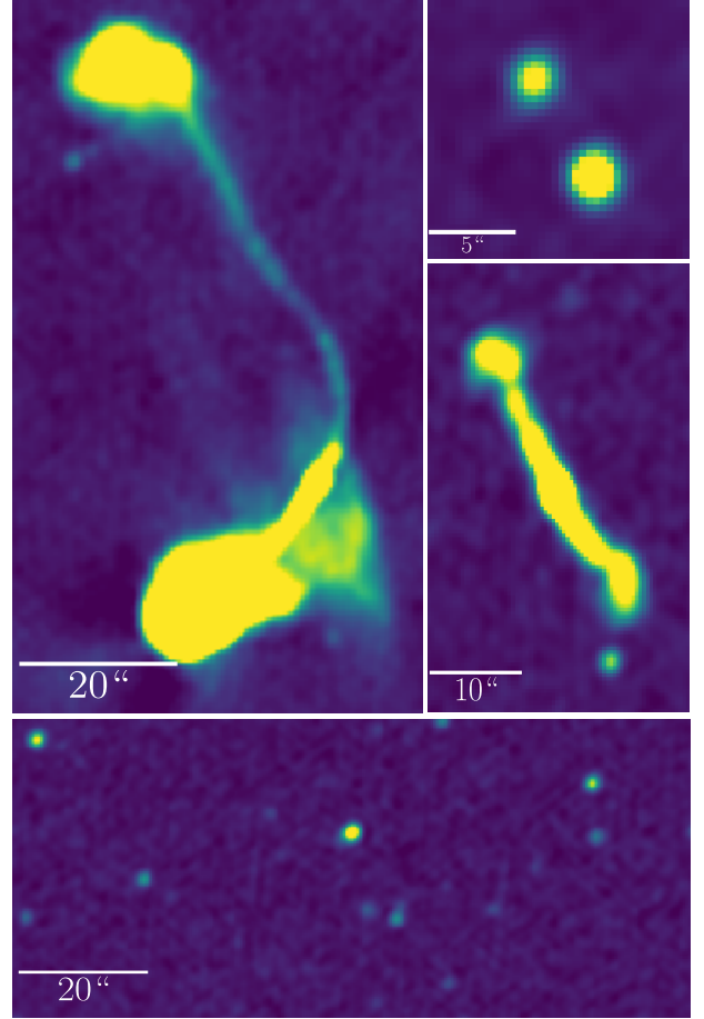
Figure 17. Stamps from the 3 GHz continuum map showing examples of extended (left and lower right image), multi-component (upper right) and compact (lower panel) radio sources. The color-scale shows the flux density from -3 \sigma_{\text{local}} to 50 \sigma_{\text{local}} , where \sigma_{\text{local}} is the local r.m.s. noise.
