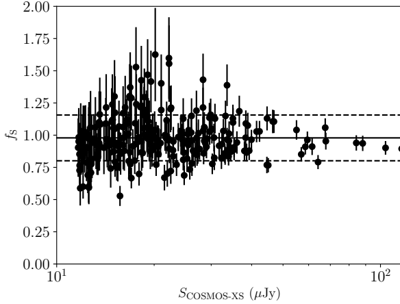
Figure 8. Flux comparison between our sample and the VLA-COSMOS 3 GHz Large Project (Smolčić et al. 2017a). The median ratio of 0.98 with a standard deviation of 0.18 shows that the flux densities are on the same flux scale.
