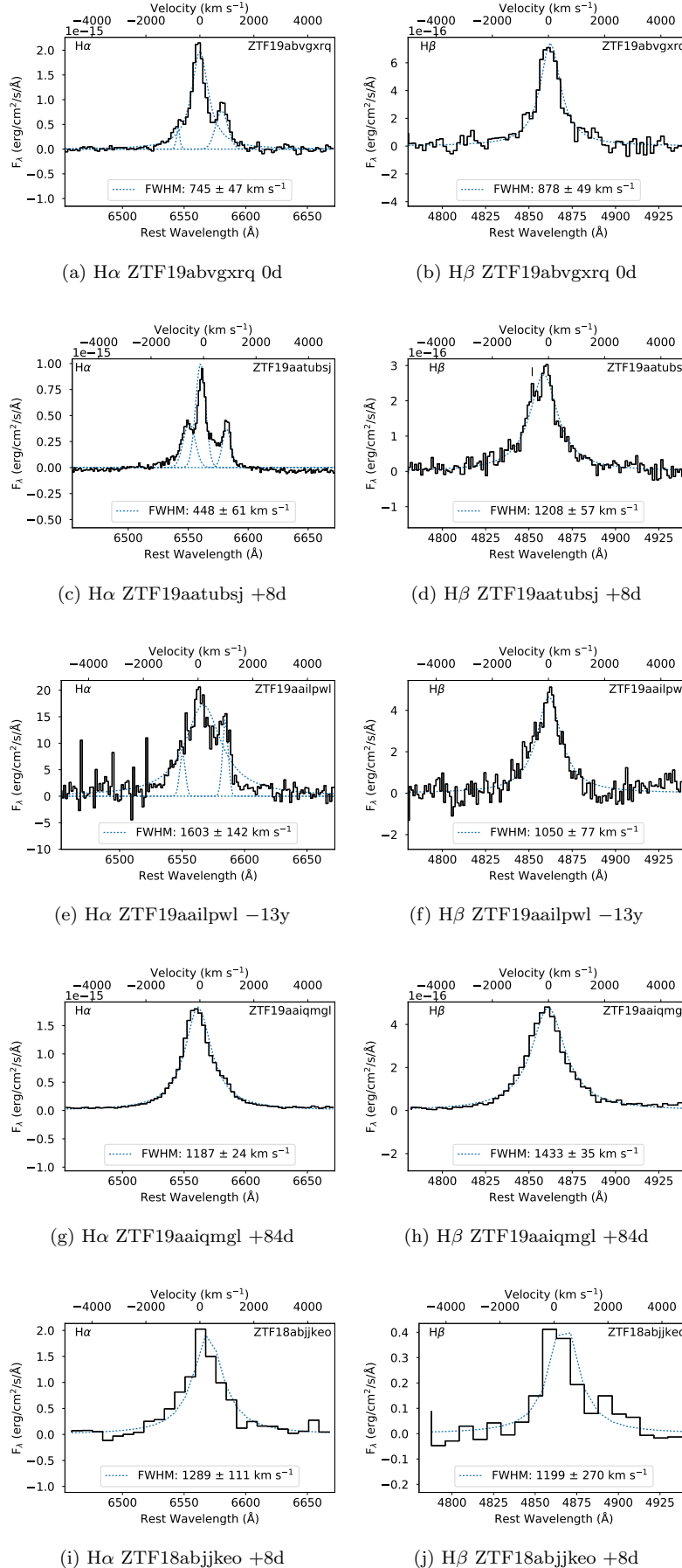
Figure 5. Gaussian fits to the H \alpha + [N II] and H \beta line profiles of all transients in the sample show that their Balmer lines have a FWHM consistent with (and Lorentzian Balmer profiles characteristic of) that of narrow-line Seyfert 1s. The offset blue peak in the H \beta profile of ZTF19aatubsj is marked by a vertical line.
