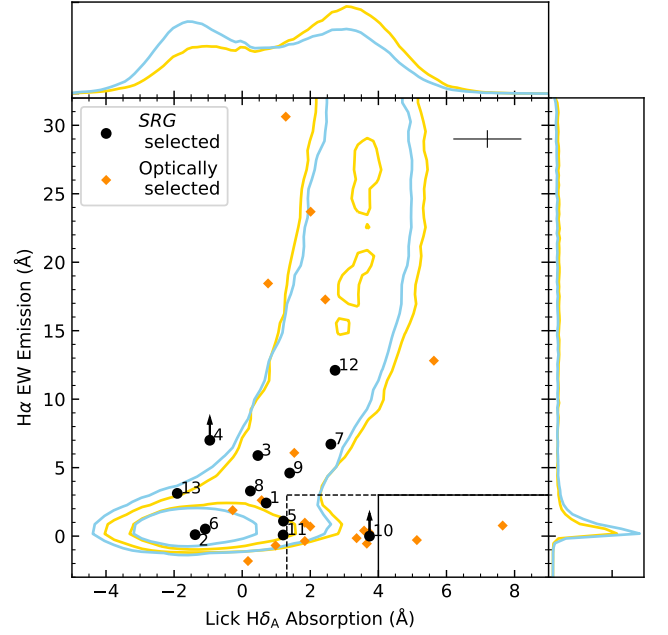
Figure 12. The H\delta_A absorption index versus the H\alpha EW emission of TDE host galaxies. The 13 black data points are from this work (labeled by their internal numbers in Table 1). The 19 orange data points are from Hammerstein et al. (2021). Median uncertainties are shown in the top right. Following the definition in Hammerstein et al. (2021), the solid black line marks the region of E+A galaxies ( H\delta_A - \sigma(H\delta_A) > 4.0 , \text{EW}(H\alpha_{\text{em}}) < 3.0 ), and the dashed black line marks the region of QBS galaxies ( H\delta_A > 1.31 , \text{EW}(H\alpha_{\text{em}}) < 3.0 ). We show two comparison samples with the distribution of M_{\text{gal}} similar to SRG selected TDE hosts (blue lines) and optically selected TDE hosts (yellow lines). For each comparison sample, the contours enclose 30% and 85% of the galaxies.
