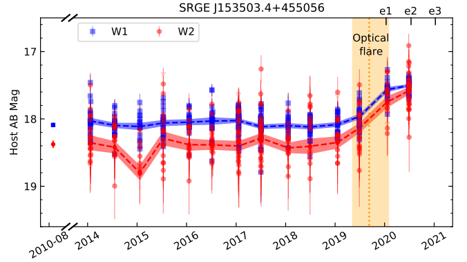
Figure 6. WISE W1 ( 3.4\mu\text{m} ) and W2 ( 4.6\mu\text{m} ) light curves of SRGE J153503.4+455056. The blue and red dashed lines mark the median magnitude of each WISE epoch. The vertical dotted line denotes the optical maximum. The vertical orange band marks the e-folding rise and decay timescales of the optical flare around the optical maximum (estimated using the Gaussian process model shown in Fig. 5). Epochs of the SRG / eROSITA visits are marked along the upper axis.
