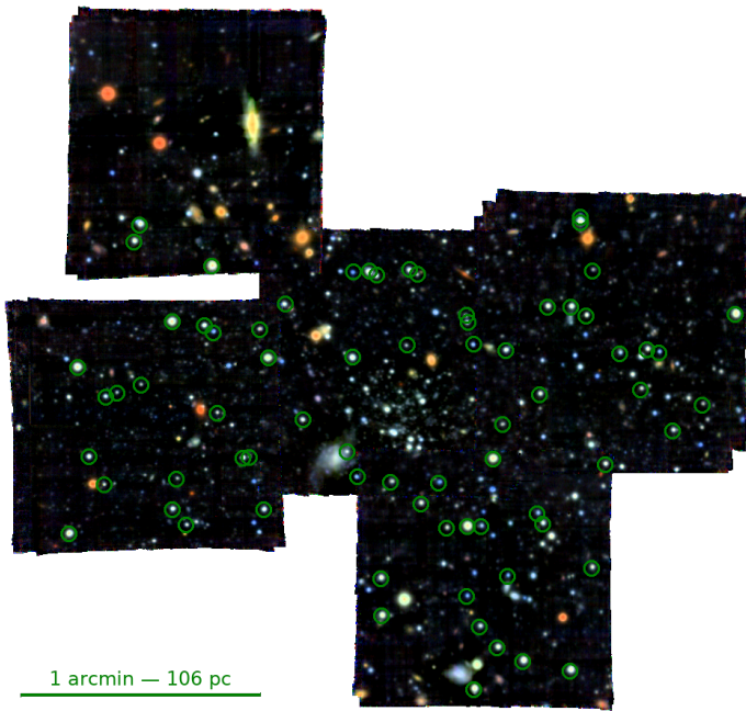
Fig. 1. Composite-colour image mosaic of Eridanus 2 as observed with MUSE-Faint. Sloan Digital Sky Survey filters g, r, and i were used for the colours blue, green, and red, respectively. Images of the five separately reduced fields were combined with Montage and the colours were composited using the algorithm of Lupton et al. (2004). The 72 member stars with MUSE-Faint measurements are circled in green. Celestial north is up. The angular and physical scale at the distance of Eridanus 2 are indicated in the bottom left corner.
