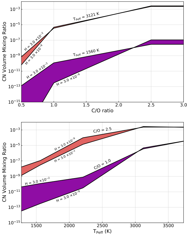
Figure 4. CN volume mixing ratio as a function of C/O ratio (upper panel) and T_{\text{Peff}} (lower panel). In the upper panel, different colours indicate different T_{\text{Peff}} . In the lower panel, different colours indicate different C/O ratios. For both panels, the spread indicates the effect of initial hydrogen abundance. The mixing ratios are averaged values of the 1.4 - 10^{-4} bar pressure region, which mostly coincides with the usual photospheric emission region. The temperature profiles used in these atmospheres are shown in Figure 1.
