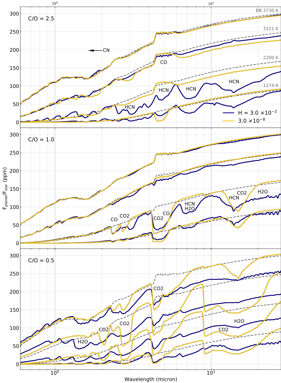
Figure 5. Synthetic emission spectra of a hot super-Earth with a nitrogen dominated atmosphere. The three panels represent three different C/O ratios (0.5 , 1.0 and 2.5). For each panel, 4 selected temperatures are shown, which coincide with the expected T_{\text{Perf}} of the planet ( T_{\text{Perf}} of 1274, 2200, 3121 and 3730 K). The blackbody emission for each of the temperatures is indicated with dashed grey lines. The spectra are shown with two different hydrogen mass fractions, indicated by colour.
