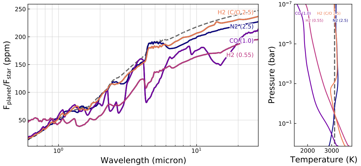
Figure 9. Comparison of synthetic emission spectra of atmospheres having different bulk compositions at T_{\text{eff}} = 3121 K. The indicated numbers in brackets represent atmospheric C/O ratio. Exact compositions are listed in the lower subsection of 1. Corresponding temperature profiles are displayed in the panel on the right.
