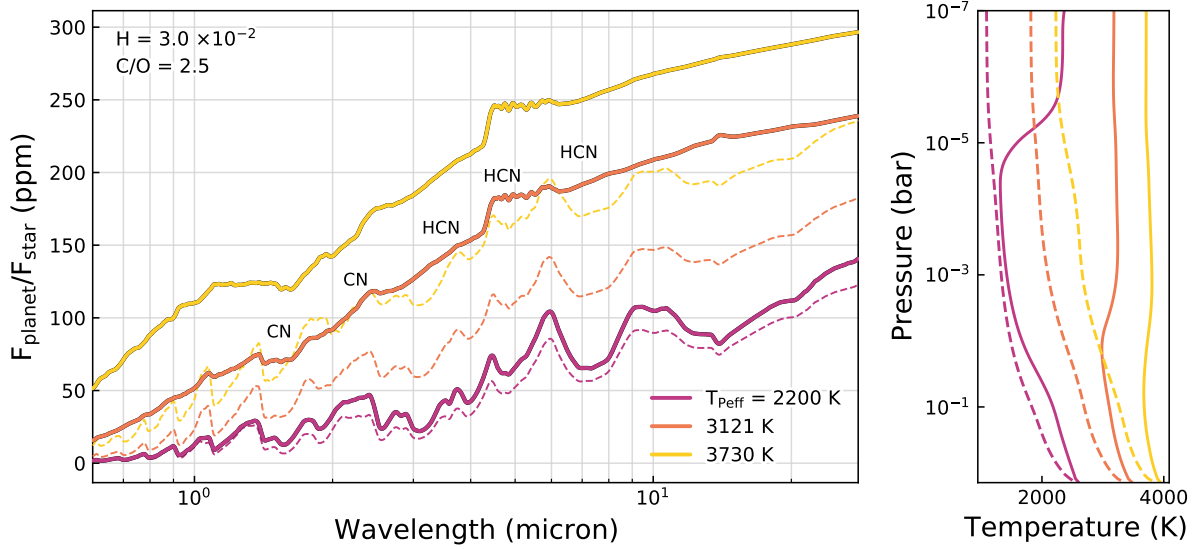
Figure 7. Comparison of emission spectra between atmospheres with strong shortwave absorbers (CN, CH, represented by solid curves) that cause temperature inversions and without (thin dashed lines). Shown for nitrogen dominated atmospheres with C/O = 2.5 , which is favourable for formation of CN (See Section 2.3). The compositions used have a hydrogen mass fraction of 3 \times 10^{-2} . Below the selected temperature range, due to inefficient CN formation, atmospheres are much less prone to temperature inversions and thus are not shown. The right panel indicates the corresponding temperature profiles.
