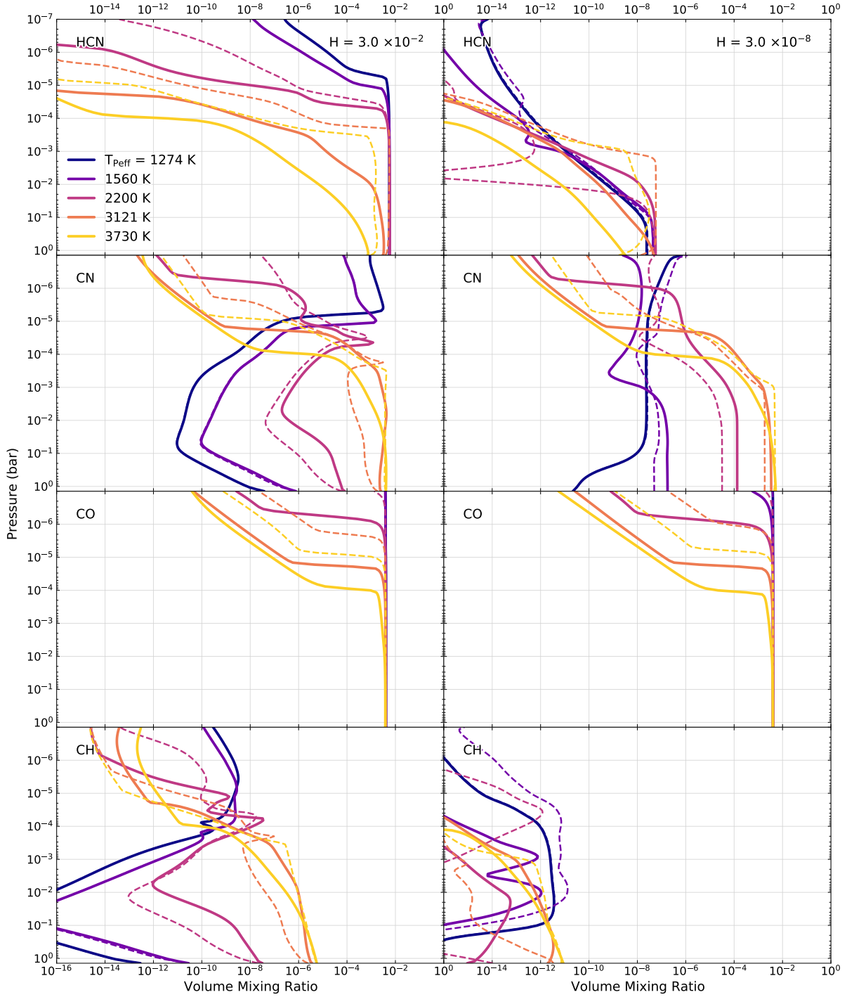
Figure 3. Volume mixing ratio of HCN, CN, CO and CH in nitrogen dominated hot super-Earth atmospheres. All cases shown for a C/O ratio of 2.5. Columns represent different hydrogen mass fractions, rows - different chemical compounds. The colour indicates the effective temperature of the planet. Solid lines represent atmospheres with temperature profiles shown in Figure 1, which in some cases have strong inversions. Dashed lines have CN and CH opacities omitted, hence lacking temperature inversions.
