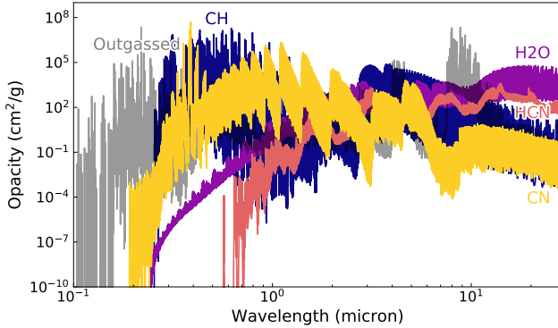
Figure 2. Opacity of CN in comparison with H 2 O, HCN and CH for T = 2900 K and P = 1 bar. Also shown is the composite opacity of an outgassed 22 mbar magma ocean atmosphere with T = 3000 K (Zilinskas et al. in prep). For each species, the opacity is calculated assuming 100% abundance and shown at a resolution of \lambda/\Delta\lambda = 1000 .
