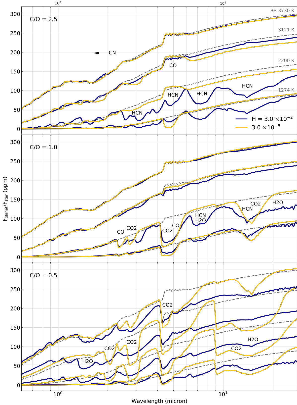
Figure 5. Synthetic emission spectra of a hot super-Earth with a nitrogen dominated atmosphere. The three panels represent three different C/O ratios (0.5, 1.0 and 2.5). For each panel, 4 selected temperatures are shown, which coincide with the expected T_{\text{Peff}} of the planet ( T_{\text{Peff}} of 1274, 2200, 3121 and 3730 K). The blackbody emission for each of the temperatures is indicated with dashed grey lines. The spectra are shown with two different hydrogen mass fractions, indicated by colour.
