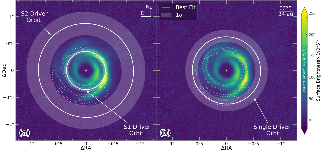
Figure 3. The best fit \pm 1\sigma orbits for assumed planetary drivers with circular orbits overlaid on ALMA contours (1.9 mm; Cazzoletti et al. 2018) and r^2 -scaled SPHERE Q_\phi image (1.2 \mu\text{m} ). (a) double-driver scenario. (b) single-driver scenario.
