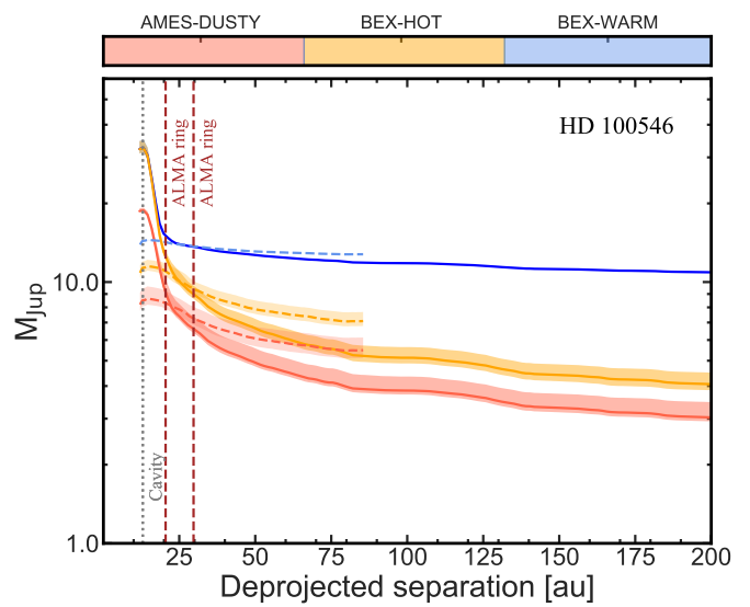
Fig. B.8. 5\sigma sensitivity to planet masses in HD 100546 (see Figure B.1).
