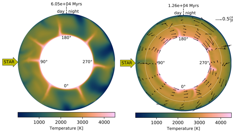
Fig. 6 Model of the geodynamic and tectonic state of the interior of LHS 3844b, assuming isothermal surface boundary conditions according to the phase maps from Kreidberg et al. (2019). The figure shows the temperature field with a weak (left) and a strong (right) surface layer, with a substellar surface temperature of 1000 K and antistellar surface temperature of 20 K. The distribution of plumes in the hemispheric tectonics regime (right) beneath the substellar point and the distribution of largely molten regions points to a tectonic regime not observed in the Solar System and may provide vital clues as to the potential variability of tectonic states across the rocky exoplanet census. Figure adapted from Meier et al. (2020).
