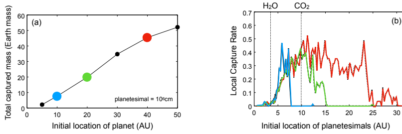
Fig. 3 Results of dynamical simulations of planetesimal capture by a migrating giant planet—The left panel shows the total mass of the planetesimals that the planet captures during its orbital migration as a function of the semi-major axis at which the planet starts migration; the right panel shows the fraction of the planetesimals located initially at an semi-major axis that the planet engulfs. The vertical dotted lines in panel (b) indicate the semi-major axes of the H 2 O and CO 2 snowlines. Those panels have been adapted from Figure 5 of Shibata et al. (2020).
