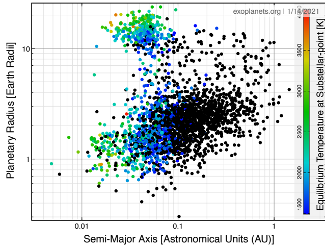
Fig. 7 Two-dimensional distribution of discovered exoplanet size and orbit. The colour contours shows the substellar-point equilibrium temperatures with zero planetary albedo larger than 1500 K. The data has been taken from an open exoplanet catalogue database ( http://exoplanets.org )
