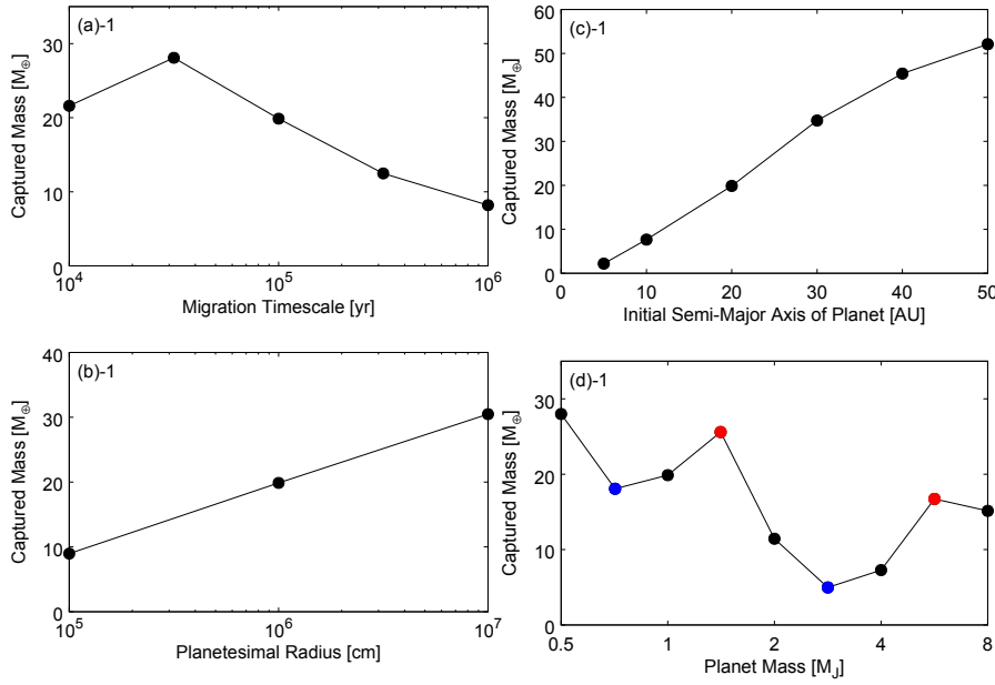
Fig. 4 Results of the parameter study of planetesimal capture by a migrating protoplanet performed by Shibata et al. (2020). Shown is the total mass of captured planetesimals in Earth masses as a function of: the migration timescale of the planet (a)-1, the radius of planetesimals (b)-1, the initial semi-major axis of the planet (c)-1, and the mass of the planet (d)-1.
