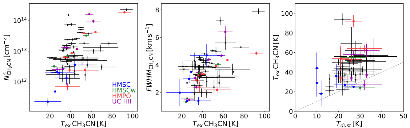
Fig. 6. Left: plot of the column densities of CH 3 CN as a function of the excitation temperature T_{\text{ex}} ; middle: plot of the FWHM of CH 3 CN as a function of the excitation temperature T_{\text{ex}} ; right: plot of the excitation temperature T_{\text{ex}} of methyl cyanide vs. dust temperature T_{\text{dust}} . The grey line indicates T_{\text{dust}} = T_{\text{ex}} .
