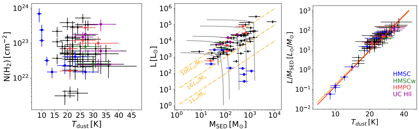
Fig. 4. Left: distribution of the sources of the sample in the plane N(\text{H}_2) - T_{\text{dust}} ; middle: distribution of the sources of the sample in the plane L - M_{\text{SED}} . Grey tracks are the evolutionary tracks from Molinari et al. (2008), while orange dashed lines indicate L/M = 1, 10, and 100 L_{\odot}/M_{\odot} ; right: plot of the color-color tracers L/M as a function of T_{\text{dust}} and power-law relation best fit to the data given in orange. The legend for the classification color-code is given in the right panel. Sources that have not been classified yet are plotted in black.
