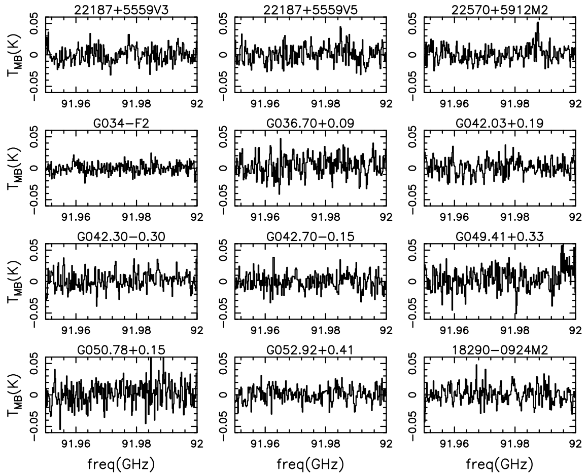
Fig. A.5 Spectra of \text{CH}_3\text{CN}(5_K-4_K) for the sources for which no transition has been detected.
