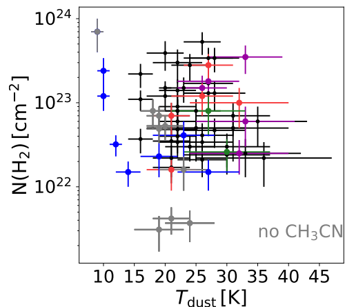
Fig. 9. Distribution of sources in the plane N_{\text{H}_2} - T_{\text{dust}} , with sources for which \text{CH}_3\text{CN} has not been detected highlighted in grey.
