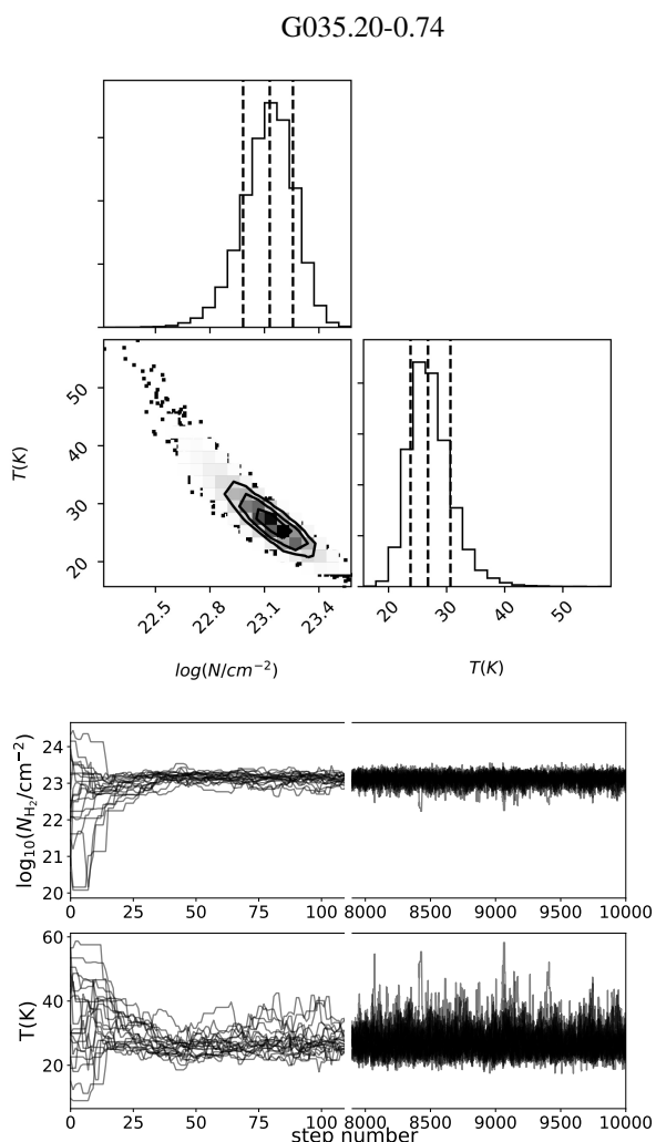
Fig. 1. Three upper panels: corner plot for the source G035.20-0.74 of the two parameters N(\text{H}_2) and T_{\text{dust}} free to vary in the MCMC used to fit the SED. The units of the y-axes of the other two panels are counts. Two lower panels: walkers of the two parameters N(\text{H}_2) and T_{\text{dust}} , for the source G035.20-0.74.
