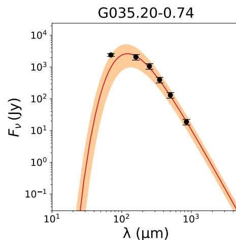
Fig. 2. SED of the source G035.20-0.74. The red line is the best fit to the SED, obtained using the parameters N_{\text{H}_2} and T_{\text{dust}} given in Table 4. The orange area represents the variation from the best fit if the two parameters are varied inside the uncertainties. The point at 70\ \mu\text{m} has not been used to constrain the fit of the SED, but it has been used to derive the luminosity of the sources.
