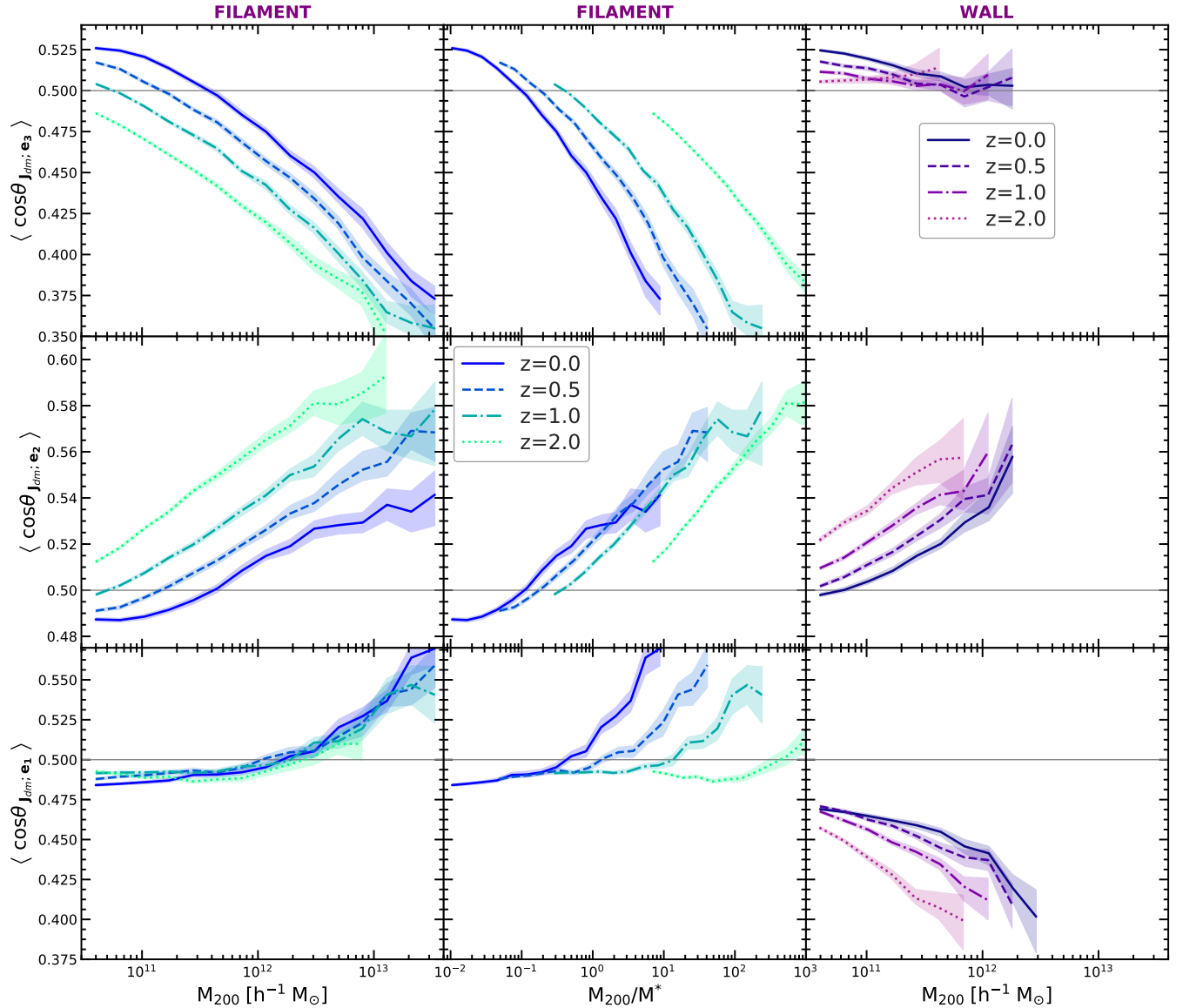
Figure 7. The evolution of halo spin alignment in filaments and walls: It shows the median alignment angle, \cos \theta , between the spins of haloes and the principal axes of their environment. The median angle is plotted as a function of halo mass (left- and right-hand columns) and halo mass normalised by the characteristic mass, M^* , at each redshift (middle column). The first two columns are for filament haloes and the right-hand column is for wall haloes. The rows correspond to three environment principal axes: \mathbf{e}_3 is the axis of last collapse (top row), \mathbf{e}_2 is the axis of second collapse (middle row), and \mathbf{e}_1 is the axis of first collapse (bottom row). The various colours and linestyles represent haloes at different redshifts, and the shaded region indicates the 1\sigma uncertainty when determining the median alignment angle.
