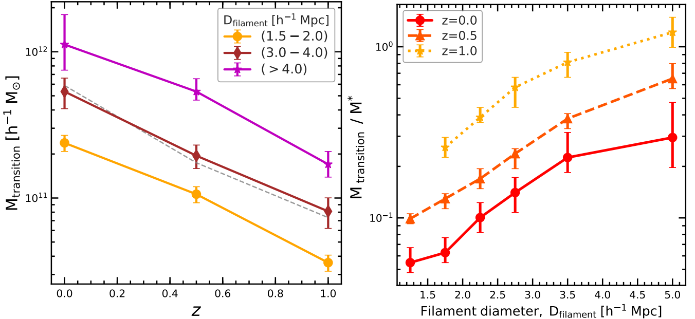
Figure 10. Transition mass and filament diameter: The left panel: shows the redshift evolution of the spin alignment transition mass for filaments of different thickness (see plot legend). The right panel: shows transition mass normalised by characteristic mass, M^* , as a function of filament diameter. The gray dashed line shows the curve (1+z)^{-3} . The transition mass increases with filament diameter and also evolves with time.
