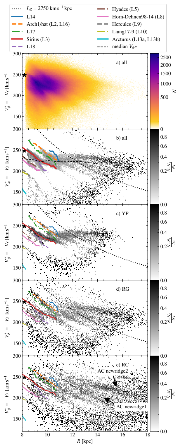
Fig. 16. Substructures in the R-V_\phi^* projection in the anticentre direction. a) Number counts in the R-V_\phi^* plane in bins of size \Delta R = 0.02 kpc and \Delta V_\phi^* = 1 km s ^{-1} for all stars in the AC20- \varpi/\sigma_\varpi > 3 sample. b) Same but applying a substructure mask to highlight the ridges (see text). c-e) Same as b but for different stellar types. We also plot: some ridges from Ramos et al. (2018) with coloured lines, the separation of the bimodality (black dotted line), and the median velocity (black dashed line in panel b). We see the ridges extending beyond their limits in DR2 and new ridges resolved here for the first time.
