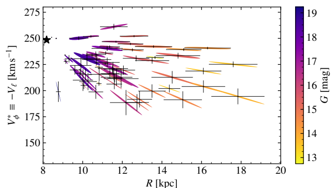
Fig. 9. Error ellipses in the R-V_\phi^* plane for stars in the anticentre. The ellipses have been drawn for 60 stars from the AC20-\varpi/\sigma_\varpi > 3 sample chosen randomly but with weight of \exp R in order to sample better the different R . The ellipses are coloured by magnitude G and the error bars are included as black lines. The error ellipses are oriented pointing towards the R_0-(v_{c,\odot} + V_\odot) point (black star).
