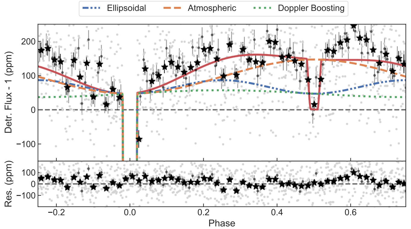
Figure 22. The phase-folded TESS SAP light curve for TOI-1431 b, zoomed in to show the phase curve and secondary eclipse, similar to Figure 11.
