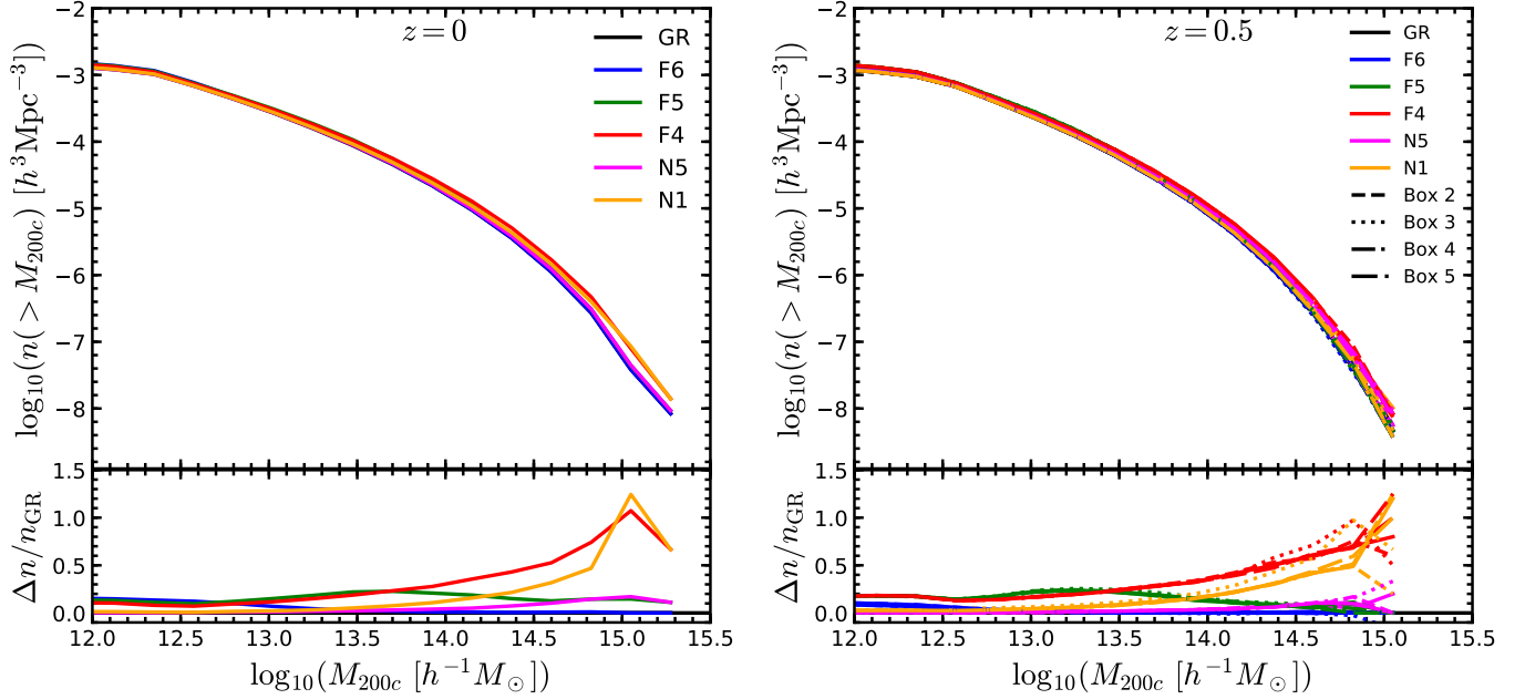
FIG. 2. (Color Online) The cumulative halo mass function for the various models simulated here, at z = 0.0 (left panel) and z = 0.5 (right panel). The bottom panels show the relative difference between the various modified gravity models and \Lambda CDM. For the z = 0.5 plot we have used all 5 realizations, and it shows that the model differences are not sensitive to the specific realization. For the z = 0 plot we only used Box 1. The line colors and styles are the same as in Fig. 1.
