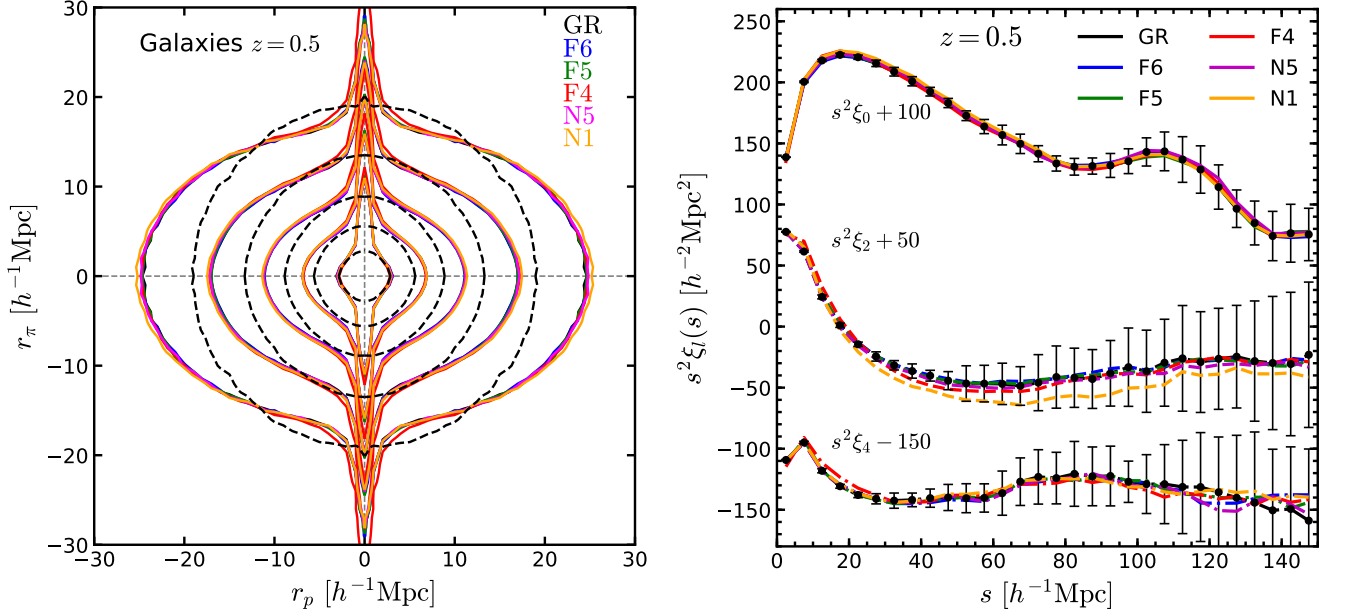
FIG. 5. Left panel: The two dimensional galaxy correlation function \xi(r_p, r_\pi) measured from our mock catalogues at z = 0.5 as a function of separation across ( r_p ) and along ( r_\pi ) the line-of-sight. Contours show lines of constant \xi(r_p, r_\pi) at \xi(r_p, r_\pi) = 5, 2, 1, 0.5, 0.25 . The correlation functions correspond to the average of fifteen measurements obtained by projecting five realizations over the three LOS directions. The black dashed contours correspond to the real-space measurements of the correlation function at the same values of its counterpart in redshift-space, for simplicity we show the GR case only for these contours. Right panel: Monopole, quadrupole and hexadecapole moments of the correlation function, Eq. (22), for our six gravity models at z = 0.5 . The moments have been shifted by a factor of 100, 50 and -150 for better visualization. The error bars correspond to the standard deviation over fifteen GR measurements. Different colour line correspond to different gravity model as specified in the legend.
