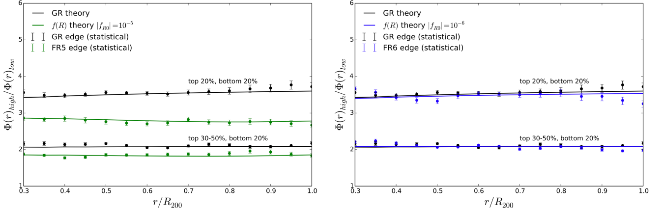
FIG. 27. The z = 0 gravitational potential ratio between high and low mass bins (of 20 halos) for GR (black), and the F5 (left) (green) and F6 (right) parametrization of modified gravity (blue). The points are the averages of the square of the measured radial escape velocities using the simulation particles for each bin in radius and mass. The errors are 1\sigma on the mean from boot-strap re-sampling. The solid lines represent the theoretical predictions using the NFW density parameter. The separation between GR and f(R) potential ratios increases with increasing separation in the mass bins and we show two different mass binning schemes in each panel where the percentages denote the percentiles of cluster masses we keep in the sample. Note the large difference between the GR and F5 ratios at either mass binning scheme. Note the precise and accurate agreement between the theory and the measured escape profile (or \Phi ) profile ratios. These figures justify our use of only theory in making predictions without the need for additional simulations at differing levels of f_{R0} .
