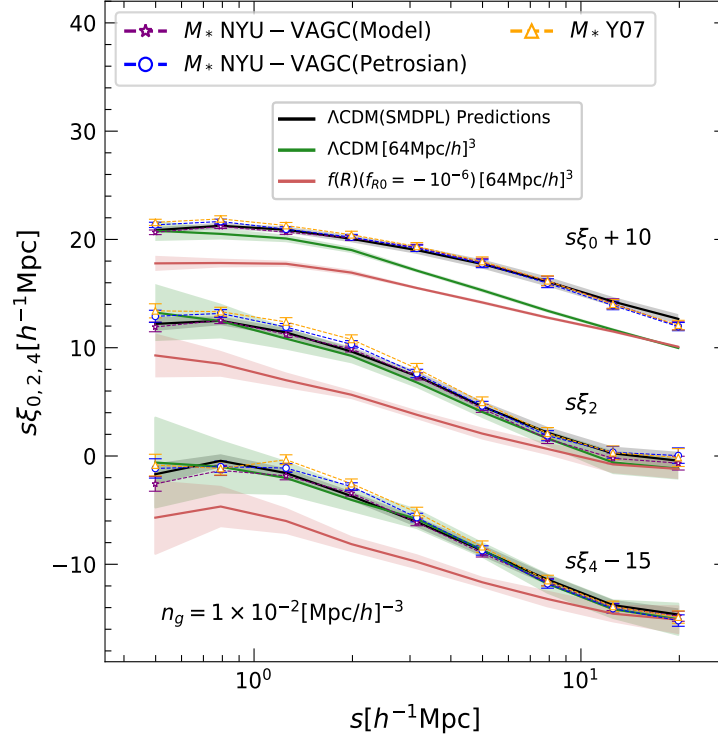
FIG. 7. A comparison of RSD measurements using three different stellar mass models: a template-fit method adopted in the NYU catalog with the SDSS model magnitude (stars with dashed line), the same template-fit method but with the SDSS Petrosian magnitude (circles with dashed lines), and a single-color method (triangles with dashed lines). Different stellar mass models give rise to convergent results. The error-bars in the above plot are estimated using a jackknife re-sampling technique with 133 realizations. Here the error-bars represent 3\sigma statistical error. The predicted RSD multipoles (monopole \xi_0 , quadrupole \xi_2 and hexadecapole \xi_4 ) in \Lambda CDM from SHAM mock are in good agreement with observations. Note that the SHAM mock is based on the SMDPL simulation [124] and has the same geometry as the real data. The plot is reproduced from [118]. The green and red lines show the predicted RSD multipoles for \Lambda CDM and f(R) gravity using a suite of simulations with 64[h^{-1}\text{Mpc}]^3 box size. The shaded regions give the 1\sigma uncertainty around the expectation value, derived from 500 realizations with line-of-sight along different directions of the simulation box. Despite the deficit of power in the monopole due to the small box size of the simulations, the higher order multipoles, such as quadrupole \xi_2 and hexadecapole \xi_4 , show significant differences, indicating that even a model like F6 can be testable given the accuracy of the clustering measurement of DESI.
