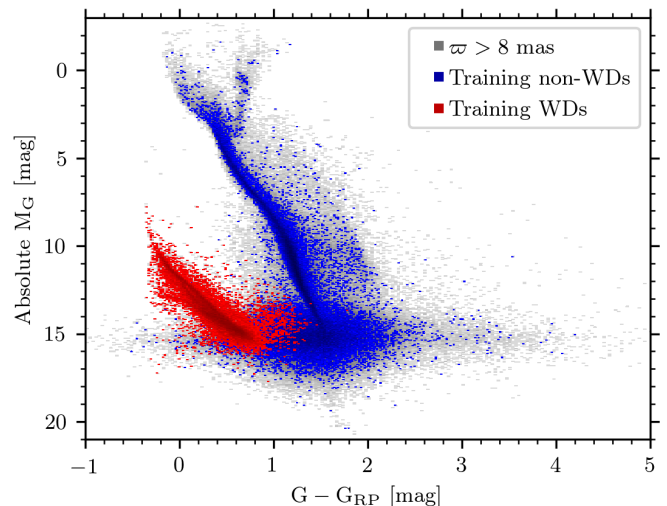
Fig. 34. CAMD for the training dataset based on which we classified the WDs. Red data points represent the WD population. Grey points are all sources in the whole \hat{c} > 8 mas sample from which these samples were extracted. The appearance of the test dataset is quite similar to the one plotted here.
