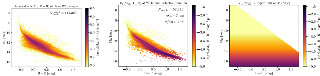
Figure 8. Comparison of the cleaned sample of likely WDs, N_C(M_G, (B - R)) (left, with units [mag -2 ]) with the modelled white dwarf LCF, \Phi_0(M_G, (B - R)) (center, with units [mag -2 pc -3 ]). The (M_G, (B - R)) domain covered by both distribution is of course the same. Yet, the density peaks of N_C(M_G, (B - R)) and of \Phi_0(M_G, (B - R)) are in dramatically different places in the (M_G, (B - R)) -plane. The reason is that the two distributions differ by the selection function integral (expressed here via V_{\text{eff}} ), which is shown in the right panel; in the case at hand the selection function ends up being only a function of M_G , not (M_G, (B - R)) ; the survey volume in the top right corner of the (M_G, (B - R)) -plane is zero, as such objects were excluded by the initial Gaia parent catalog query.
