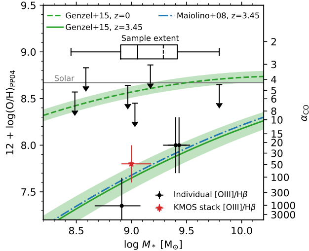
Figure 9. Plot of the mass-metallicity (MZ) relation and corresponding \alpha_{\text{CO}}(Z) (Equations 4 and 5; Genzel et al. 2015), as function of stellar mass ( M_* ). The constraints on the MZ relation at z = 3.45 come from Maiolino et al. (2008). Metallicity is plotted as 12 + \log(\text{O}/\text{H}) on the Pettini & Pagel (2004) scale. The inset shows a boxplot with the whiskers indicating the full stellar mass extent of the sample, the box the interquartile range, the solid line the median, and the dashed line the (linear) mean M_* of the sample. The black points show direct constraints ( 3\sigma limits) on the metallicity of a few galaxies via [\text{O III}] \lambda 5008/\text{H}\beta \lambda 4863 , with 0.3 dex uncertainty, using the direct method (Curti et al. 2017), conservatively assuming the upper branch solution for the upper limits. The red star shows the average metallicity from the stack of the KMOS spectra (Fig. 10) at the mean stellar mass (error bars correspond to the 16th and 84th percentile). Overall, the measurements are consistent with the MZ relation at the typical redshift of the sample.
