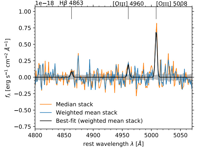
Figure 10. Stacked NIR spectra of the galaxies observed with KMOS (continuum subtracted). We show the median stack (orange), the weighted mean stack (blue, with propagated errors in gray) and the best-fit to the weighted mean stack (in black, with uncertainties). We tentatively detect \text{H}\beta \lambda 4863 , measuring \log([\text{O III}]/\text{H}\beta) \approx 0.9 \pm 0.3 , which broadly implies a metallicity of 12 + \log(\text{O}/\text{H}) \approx 7.6 - 8.0 (Curti et al. 2017).
