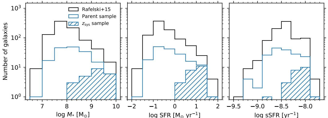
Figure 2. Histograms of the stellar mass ( M_* ), star formation rate (SFR) and specific SFR ( sSFR = SFR/M_* ) of the galaxies for which we determine a systemic redshift ( z_{\text{sys}} ), compared to the parent sample from MUSE at 3.0115 \leq z < 3.812 and all galaxies from the photometric redshift catalog by Rafelski et al. (2015).
