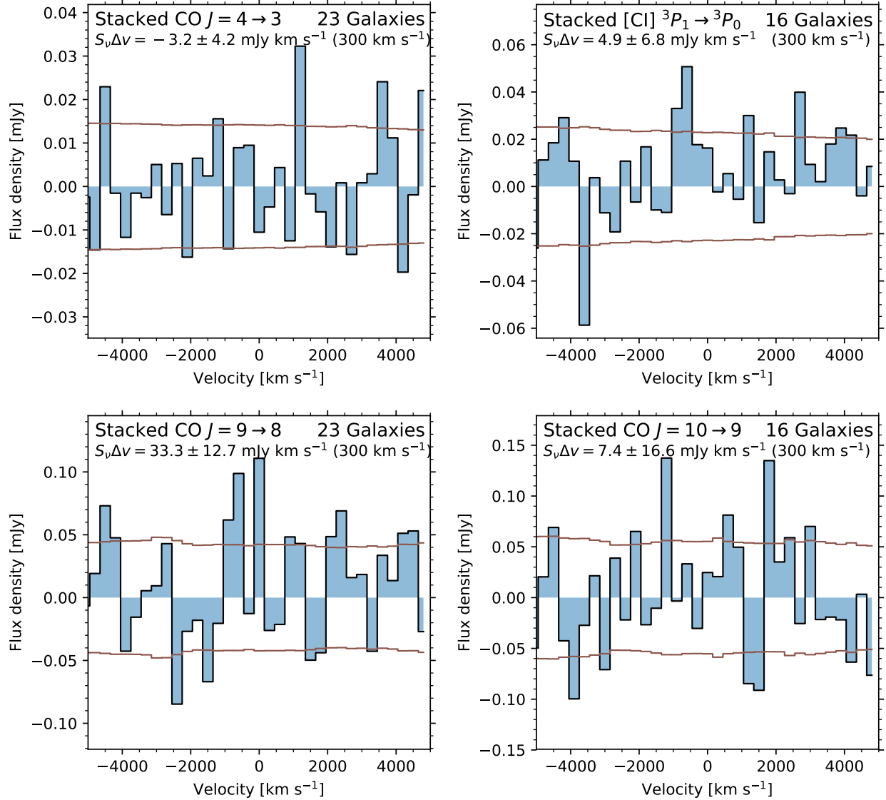
Figure 6. Stacked spectra of the ^{12}\text{CO} and [\text{C I}] transitions of the full sample. The spectrum is shown in blue and the brown line shows the root-mean-square noise (propagated through the 1/\sigma^2 -weighting of the stack). The stacked transition, the number of galaxies in the stack, the integrated line flux in the zero-velocity channel and the channel width ( 300 \text{ km s}^{-1} ) are indicated in each panel. We do not detect any emission in any of the transitions and provide 3\sigma upper limits in Table 1.
