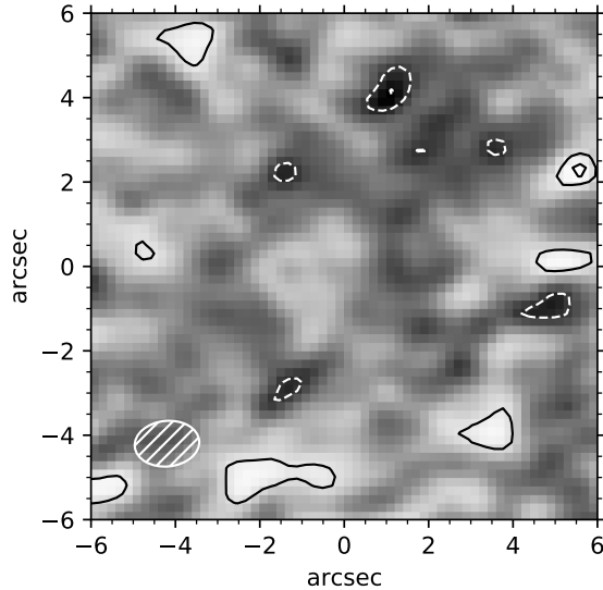
Figure 7. Stack of the 1.2 mm dust continuum. The cutout size is 12'' \times 12'' and the synthesised beam is indicated in the bottom left corner. Contours are drawn starting at \pm 2\sigma in steps of \pm 1\sigma (dashed contours indicate negative signal). No emission is detected at the 3\sigma level, implying an upper limit of 9 \mu\text{Jy} .
