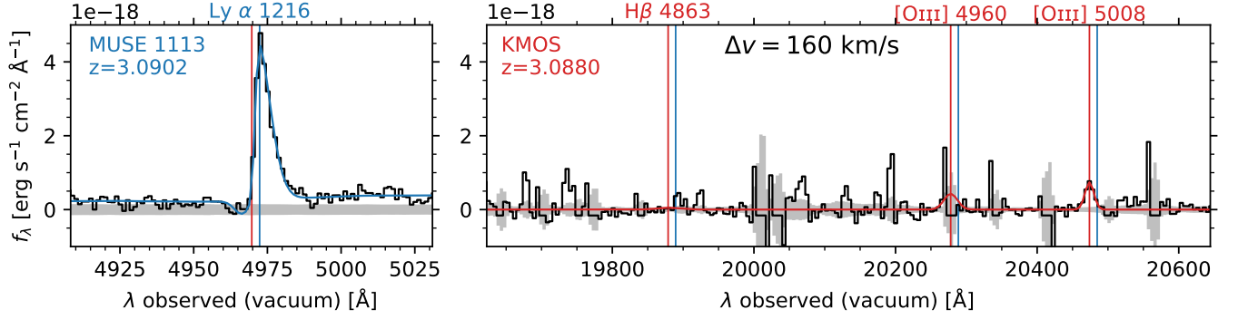
Figure 3. Rest-frame ultraviolet and optical spectra for the first galaxy in the sample with near-infrared follow-up. The left panel shows the MUSE spectrum surrounding the Ly \alpha line. The right panel shows the continuum subtracted KMOS spectrum around the H \beta \lambda 4863 and [O III] \lambda\lambda 4960, 5008 lines. In both panels the vertical blue and red lines indicate the redshift of Ly \alpha and the systemic redshift, respectively, determined from the fit to the spectrum (shown in the same color). This particular galaxy is detected in Ly \alpha \lambda 1216 and [O III] \lambda 5008, but not in H \beta \lambda 4863, showing a positive velocity offset between the red peak of Ly \alpha and the systemic redshift (note [O III] \lambda 4960 falls on top of a skyline). Spectra of the remaining galaxies with KMOS or MOSFIRE observations are shown in Fig. 12 in Appendix A.
