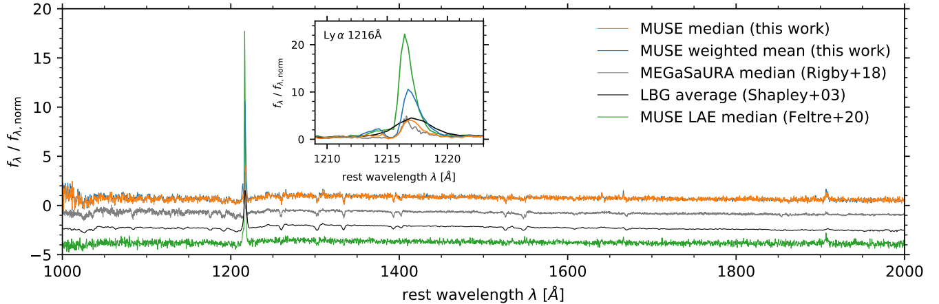
Figure 4. Composite MUSE spectrum of the sample, from both weighted mean (blue) and median (orange) stacking (at 0.3 Å resolution) using the systemic (non- \text{Ly}\alpha ) redshifts. We compare to the average Lyman Break Galaxy (LBG) spectrum at z \sim 3 (black) from (Shapley et al. 2003, 1 Å resolution), the composite spectrum of 14 strongly lensed, star-forming galaxies at 1.6 < z < 3.6 from the MEGaSAURA sample (Rigby et al. 2018; the pivot normalized, median stack at 0.1 Å resolution) and the composite MUSE spectrum of all 220 LAEs at 2.9 < z < 4.6 (Feltre et al. 2020, median stack; note their weighted mean stack is very similar, with slightly stronger \text{Ly}\alpha emission). We normalize all spectra to the median flux density at 1267–1276 Å and offset the literature spectra by -1.5 , -3 and -4.5 for clarity. The inset shows a zoom-in of the \text{Ly}\alpha -line without vertical offsets. Overall, the composite MUSE spectrum is very similar to the LBGs and MEGaSAURA, showing comparable UV continuum and absorption features, slightly stronger UV emission lines, and a comparable strength of the \text{Ly}\alpha -line in the median spectrum (notably showing a blue bump). In contrast, the median stack of all LAEs from Feltre et al. (2020) shows significantly stronger \text{Ly}\alpha -emission, even when compared to the weighted mean spectrum of our galaxies.
