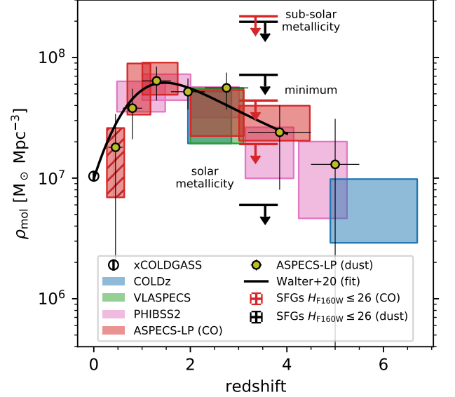
Figure 11. Cosmic molecular gas density as a function of redshift. The literature data is from Fletcher et al. (2020) (xCOLDGASS), Riechers et al. (2019) (COLDz), Riechers et al. (2020) (VLASPECS), Lenkić et al. (2020) (PHIBSS2), Decarli et al. (2020) (ASPECS-LP CO), Magnelli et al. (2020) (ASPECS-LP dust) and we also show the best-fit from Walter et al. (2020). We show the estimates on the upper limit on the cosmic molecular density for all galaxies with H_{\text{F160W}} \leq 26 at 3.0115 < z < 3.812 , as derived from CO (red; assuming r_{41} = 0.5 ) and the dust-continuum (black), under the assumption our stacked averages are representative for the larger population. The different limits are for conversion factors (\alpha_{\text{CO}}, \delta_{\text{GDR}}) = (4.36, 100) , (10, 1200) , (50, 3300) , corresponding to solar metallicity, the minimum value based on § 4.2, and the best-estimate sub-solar metallicity (the CO-based literature data is scaled to match our assumption on \alpha_{\text{CO}}^{\text{MW}} ). The upper limits do not rule out a large amount of molecular gas in lower mass galaxies (that would have been missed in previous surveys, due to their high gas mass-to-light ratio), but are equally consistent with a smaller contribution to the total molecular gas budget.
