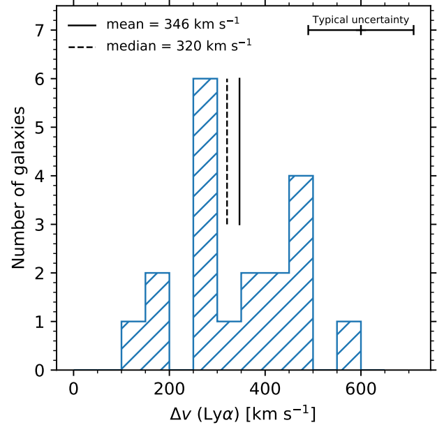
Figure 5. Histogram of the velocity offset of Ly \alpha 1216 with respect to the systemic redshift, \Delta v(\text{Ly}\alpha) . The vertical lines indicate the mean and median velocity offset in the sample. The typical \pm 1\sigma -uncertainty on the velocity offset is indicated in the top right.
