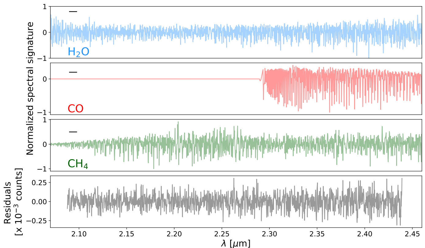
Fig. 2: Molecular templates after removal of the continua ( \text{H}_2\text{O} in blue, \text{CO} in red and \text{CH}_4 in green) and residuals of the data at the position of the planet (grey). No broad feature is visible and only individual absorption lines at the instrument resolution are cross-correlated. The small black dashes in the top left of the first three panels represent the filter size for continuum removal. Features smaller than this are kept in the residuals, while larger structures are removed as part of the continuum.
