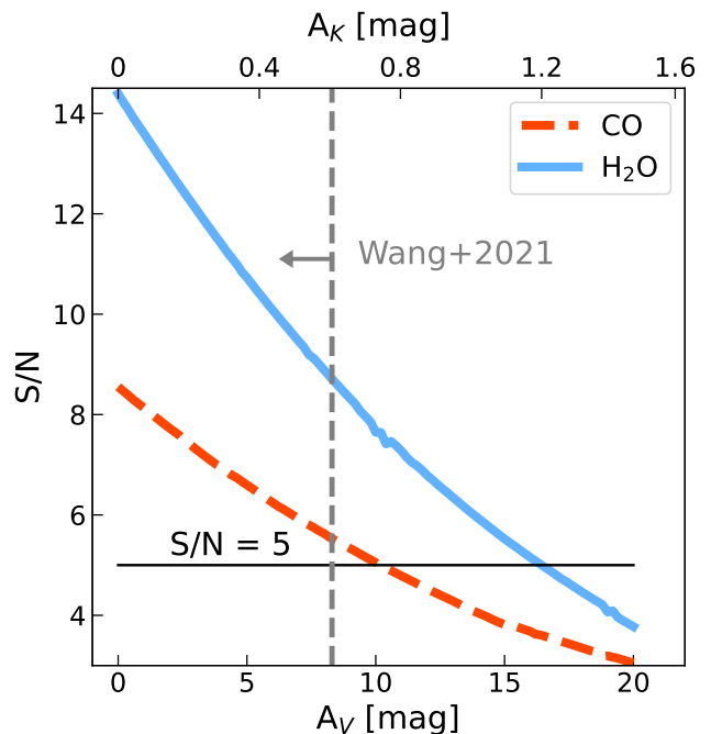
Fig. 5: Signal to noise ratio of the detection of \text{H}_2\text{O} and \text{CO} as a function of extinction affecting the emission spectrum of the planet. Assuming PDS70 b has the same chemical composition as HR8799 c, an additional extinction with A_V \approx 16 - 17 mag ( A_K \approx 1.2 mag, using the extinction law from Wang & Chen 2019) is required in order not to detect molecules with S/N > 5 . The vertical dashed line shows the maximum value obtained by SED fitting from Wang et al. (2021). Such an extinction would have revealed molecules in the planet atmosphere with S/N \sim 7-9 .
