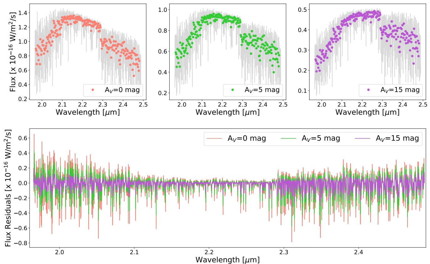
Fig. 7: Top: Extincted best-fit BT-Settl models resampled at the SINFONI (grey) and at the GRAVITY (colored circles) spectral resolution. Even with high extinction, the broad-band absorption features at the edges of the K -band spectrum can be identified. Bottom: Spectral features at the SINFONI resolution after the removal of the continuum. Higher extinctions decrease the spectral signatures molecular mapping is looking for, impeding the detection of molecules.
