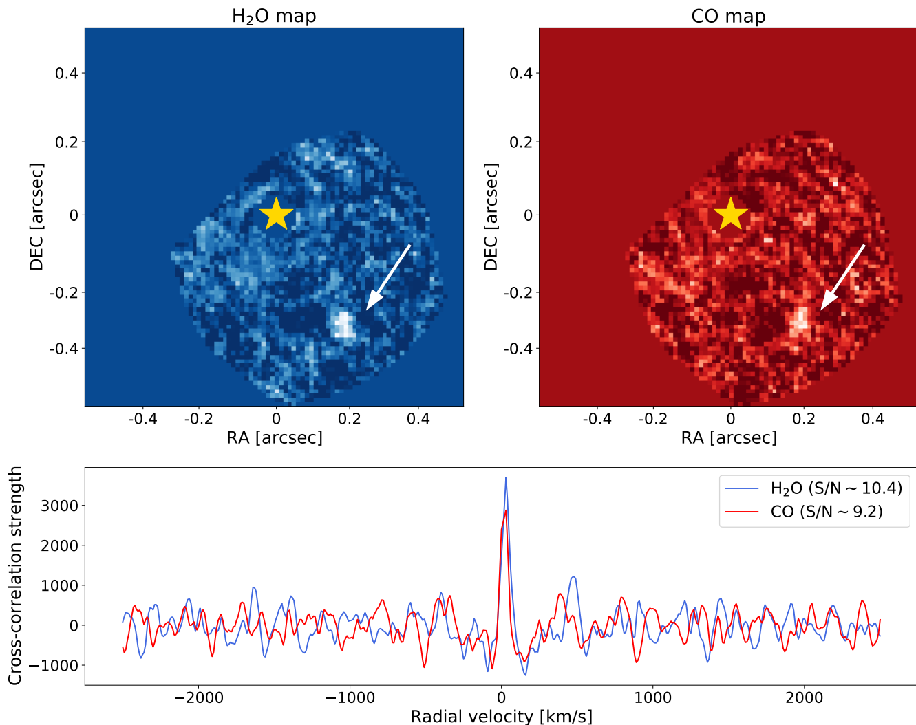
Fig. A.2: Top: Molecular maps for H 2 O and CO obtained from a dataset of \beta Pic published in Hoeijmakers et al. (2018) . North is pointing to the top, East to the left. Bottom: Cross-correlation function extracted at the planet position. The peaks representing the detection of water and carbon monoxide are clearly visible.
