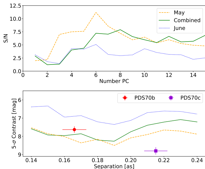
Fig. A.1: Top: S/N of PDS70 b for the first dataset (orange dashed line), the second one (blue dotted line) and the combination of the two (green solid line) as a function of the number of removed principal components. Bottom: Contrast curves obtained for the three considered datasets. Colors and linestyles are the same as in the top panel. PDS70 b separation and contrast estimates (see App. B) is marked as a red square. PDS70 c position and contrast are taken from Haffert et al. (2019).
