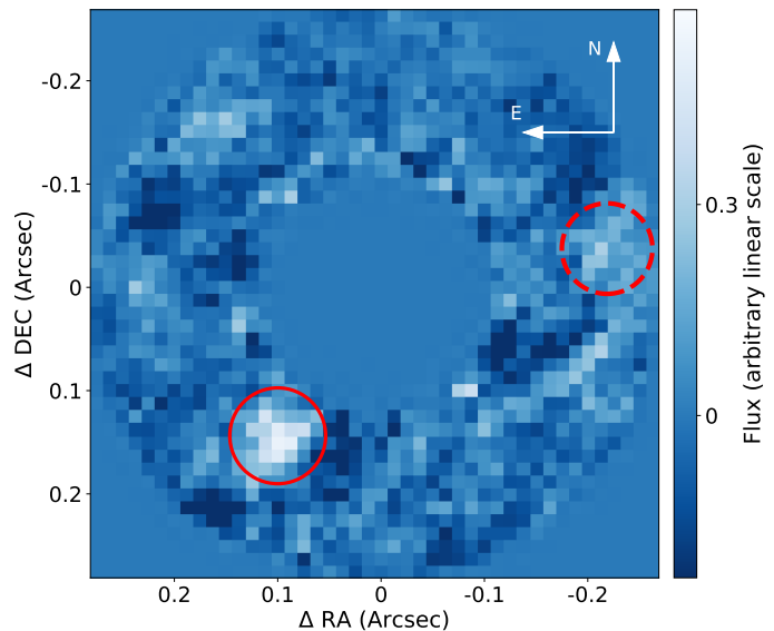
Fig. 1: Left: PDS70 system with the b planet shown in the red solid circle. Six principal components were removed from the first dataset to detect the planet with S/N \sim 12 . The dashed circle shows the expected position of PDS70 c ( Mesa et al. 2019 ).
