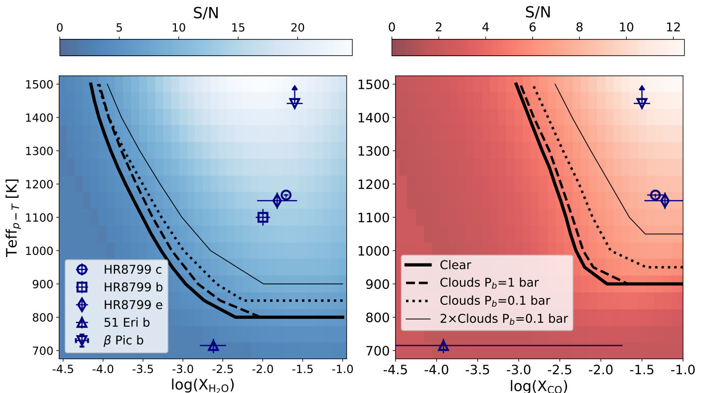
Fig. 4: H 2 O (left) and CO (right) detection maps for clear atmospheres as a function of mass fraction X_{\text{mol}} and effective temperature T_{\text{eff},pT} of the planet. Markers represent measured values for other directly imaged companions. Thick solid lines separate the region with S/N > 5 from regions with S/N < 5 , i.e., represent the molecular detection limit as a function of planet temperature. Dashed, dotted and thin solid lines represent the molecular detection limits for different cloud configurations based on Mollière et al. (2020) as described in the main text ( P_b = 10^{-3} bar is not shown). PDS70 b’s temperature ranges between 1200 and 1400 K (Stolker et al. 2020a; Wang et al. 2021). The effective temperature of \beta Pic b is well constrained as T_{\text{eff}} = 1742 \pm 16 K (Gravity Collaboration et al. 2020) and the arrow in its marker indicates that it is higher than the maximum T_{\text{eff},pT} considered here and should not be interpreted as a lower limit.
