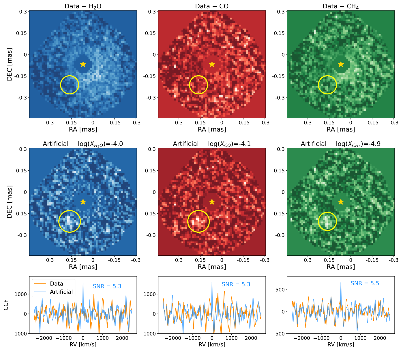
Fig. 3: Top row: H 2 O, CO and CH 4 molecular maps of the PDS70 system at RV \sim -5 km/s. The central star represents the position of PDS70 A, while the yellow circle indicates where a signal from PDS70 b should be found. Middle row: Same as in the top row, but a planet with the molecular abundances indicated on the top of each panel has been inserted in the data and detected with S/N \sim 5. Bottom row: CCF as a function of the radial velocity at the location of the planet. The orange lines represent for each molecule the CCF of the data, while the blue ones the CCF of the inserted artificial planets.
