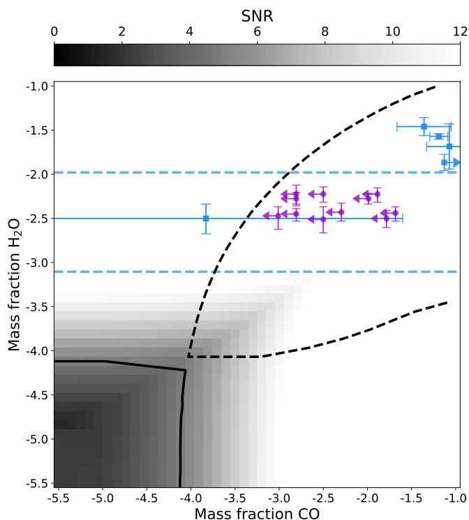
Fig. 6: Comparison of the detectability of molecules in the SINFONI data with measured abundances from substellar objects. Blue squares represent directly imaged companions HR8799 bce, \beta Pic b and 51 Eri b (Lavie et al. 2017; Wang et al. 2020a; Mollière et al. 2020; Gravity Collaboration et al. 2020; Whiteford et al. 2020, submitted) while blue lines show the measured range for H 2 O in \kappa And b (Todorov et al. 2016). The blue arrow indicates the measured value was higher than the range of abundances shown in the plot. Violet circles represent a sample of T-dwarfs analyzed in Line et al. (2017). In this case arrows refer to upper limits. The solid black line represents the region where no molecule would have been detected in our SINFONI data because of too low mass fractions. Conversely, the dashed black line encloses the region where both molecules would have been detected.
