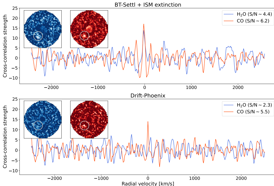
Fig. 8: Cross-correlation function for injected planets emitting as the BT-Settl+ISM extinction (top) and DRIFT-PHOENIX (bottom) best fit models proposed in Wang et al. (2021). CO is detected in both cases, while H 2 O only in the BT-Settl model. S/N of each detection are reported in the legends. The insets on the top left of each panel show the detection maps for H 2 O (blue) and CO (red).
