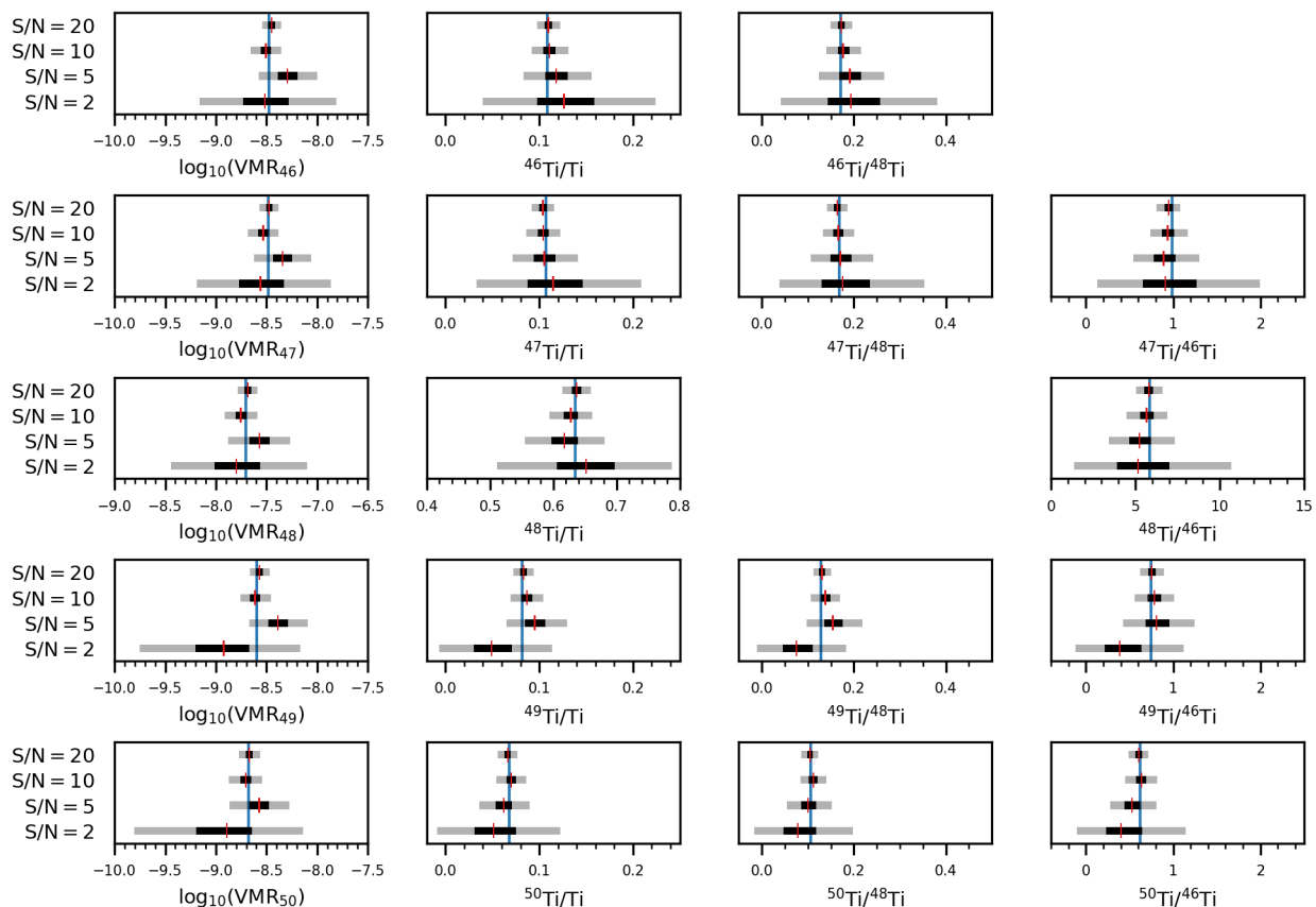
Fig. 3. Same as Fig. 2, but for the MCMC retrievals of TiO features in the narrow, broadband-filtered CARMENES spectrum of GJ 1002 with various levels of noise added. The results from the retrieval of the narrow/broadband-filtered spectrum without added noise are shown by the vertical blue lines.
