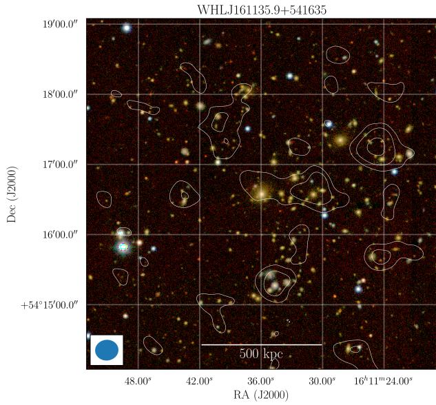
Fig. 21: Optical ( grz ) image of WHLJ161135.9+541635 from the Legacy Survey with compact source subtracted low-resolution LOFAR contours overlaid. The beam size is 20'' \times 18'' . Contours at [3, 6, 12, \dots]\sigma , where \sigma = 62 \mu\text{Jy beam}^{-1} .
