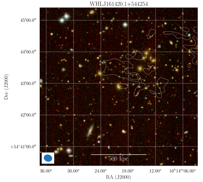
Fig. 22: Optical ( grz ) image of WHLJ161420.1+544254 from the Legacy Survey with compact source subtracted low-resolution LOFAR contours overlaid. The beam size is 16'' \times 13'' . Contours at [3, 6, 12, \dots]\sigma , where \sigma = 66 \mu\text{Jy beam}^{-1} .
