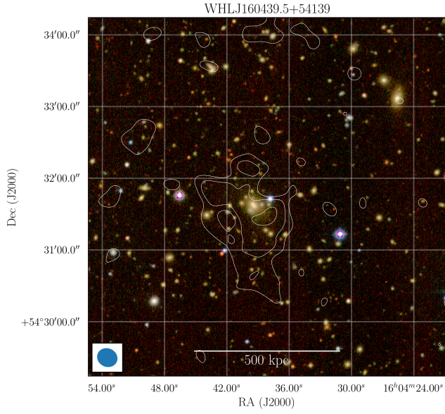
Fig. 20: Optical ( grz ) image of WHLJ160439.5+54139 from the Legacy Survey with compact source subtracted low-resolution LOFAR contours overlaid. The beam size is 17'' \times 15'' . Contours at [3, 6, 12, \dots]\sigma , where \sigma = 72 \mu\text{Jy beam}^{-1} .
