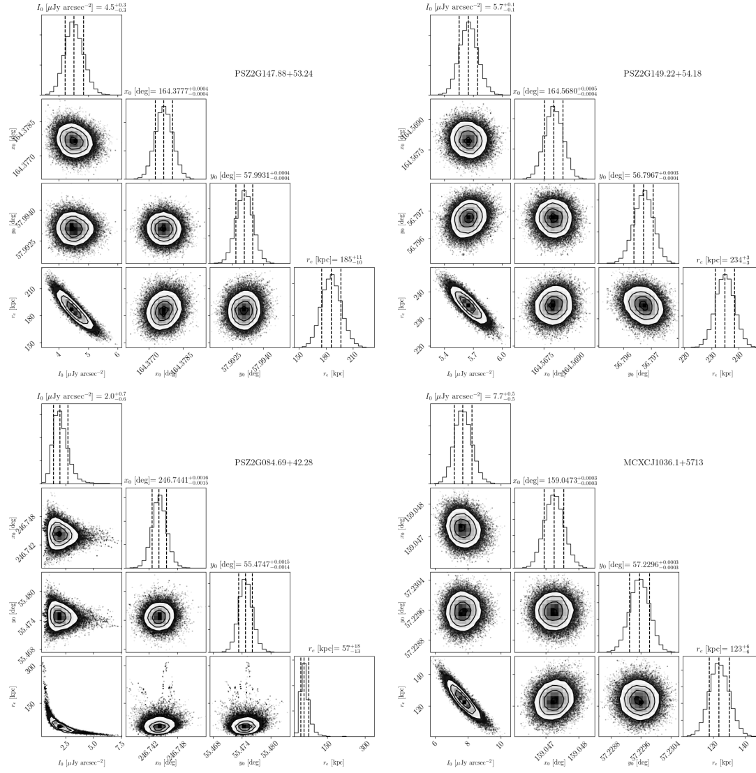
Fig. 19: Corner plots of the fitted parameters given by the MCMC chain. The dashed lines indicate the 16, 50th and 84th percentiles of the chain and the solid line indicates the initial value found by a least-square fit.
