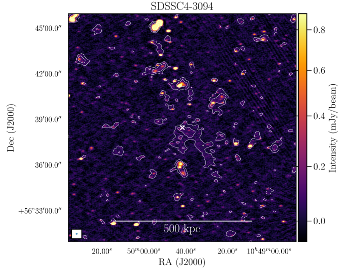
Fig. 9: SDSSC4-3094 LOFAR radio intensity map with a restoring beam of 9'' \times 5'' , with low-resolution ( 21'' \times 19'' ) compact source subtracted contours showing diffuse emission at [3, 6, 12..]\sigma , where \sigma = 74\mu\text{Jy beam}^{-1} . The white cross marks the location of the brightest cluster galaxy.
