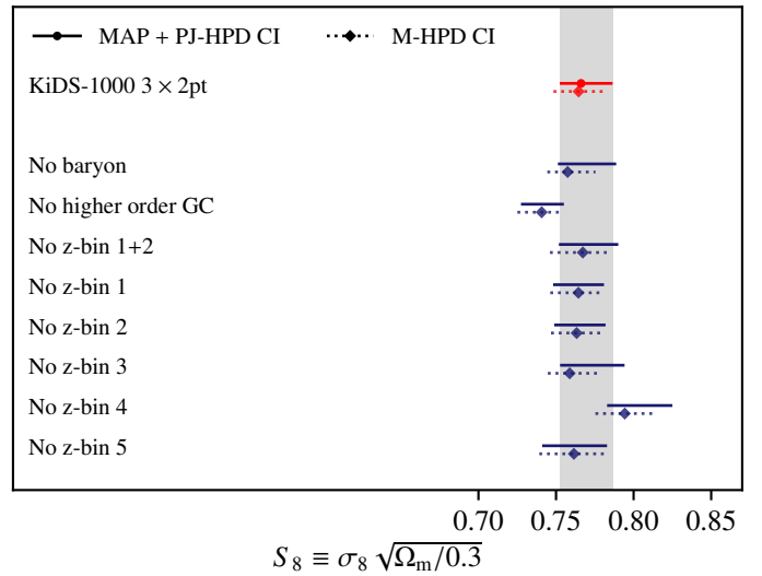
Fig. 7: 3 \times 2 pt constraints on S_8 for a series of sensitivity tests; when we ignore the impact of baryon feedback (the ‘No baryon’ case), limit the analysis to a linear galaxy bias model (the ‘No higher order GC’ case), and remove individual tomographic bins from our weak lensing observables.
