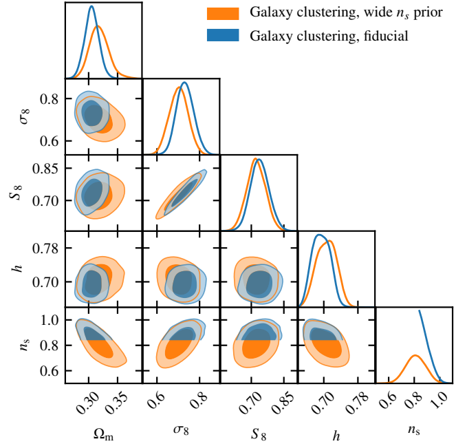
Fig. B.1: The impact of the n_s prior: Comparing marginalised posterior distributions for the BOSS galaxy clustering analysis for our fiducial analysis (blue) with the constraints when adopting an uninformative prior on n_s (orange). Opening the parameter space to arguably unphysical values of n_s favours higher values and weaker constraints on \Omega_m . Constraints on S_8 are, however, fairly insensitive to the choice of n_s prior.
