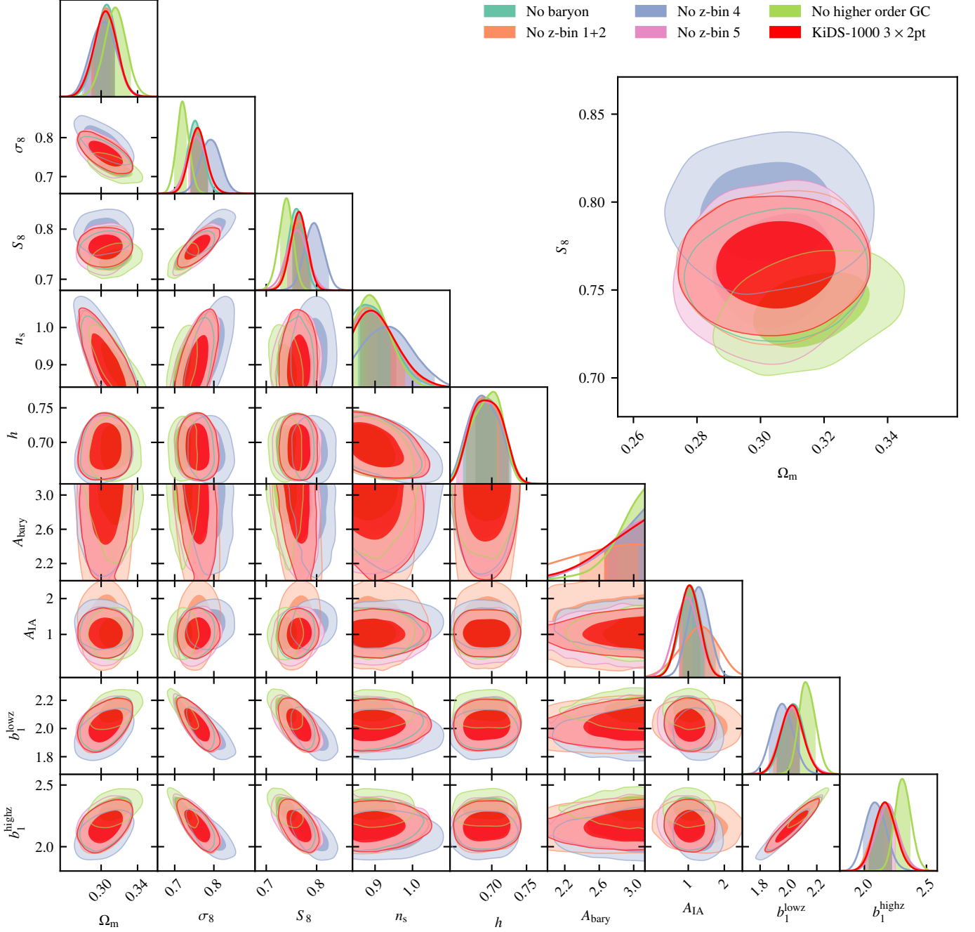
Fig. D.1: Marginalised posterior distributions for the extended set of cosmological parameters shown in Fig. 6, comparing the fiducial 3 \times 2 pt analysis (red) to a selection of our sensitivity test analyses where we ignore the impact of baryon feedback (the ‘No baryon’ case, sea-green), limit the analysis to a linear galaxy bias model (the ‘No higher order GC’ case, lime-green), and remove individual tomographic bins from our weak lensing observables (orange, purple and pink).
