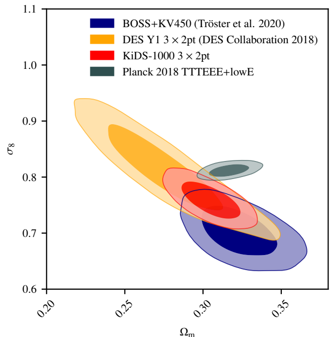
Fig. 8: Marginalised posterior distribution in the \sigma_8 - \Omega_m plane, comparing the 3 \times 2 pt analyses from KiDS-1000 and DES Y1 (Abbott et al. 2018) with the CMB constraints from Planck Collaboration et al. (2018). The KiDS-1000 3 \times 2 pt result can also be compared to our previous KV450-BOSS analysis from Tröster et al. (2020).
