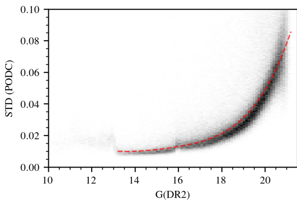
Fig. 15. Standard deviation of the PODC per-transit photometry (in magnitudes), as a function of Gaia DR2 magnitude. We overlay a fourth-order polynomial model, fit to the median standard deviation as a function of G_{\text{DR2}} magnitude.
