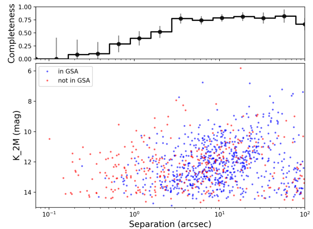
Fig. 23. Main panel: 2MASS ‘host’ galaxy magnitude (K-band) versus distance to SN (arcseconds) for those events published by GSA (in blue), and those missed (in red). Upper panel: completeness as a function of separation. We also note the likely incorrect host identification for separations greater than 30'' .
