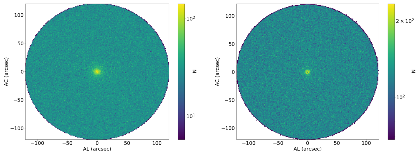
Fig. 19. The number of neighbouring sources within 2' of each published alert in the AL and AC directions at the time of the alert, accumulated for all alerts which are confirmed by ancillary data (Left), and for the remaining alerts (Right). Note that all sources within 0.2'' of the alert positions are excluded as they are deemed to belong to the alerts themselves. The distribution of sources around the alerts shows no excess in the AL and AC directions, as might be expected were there some residual contamination due to the PSF spikes of bright stars causing false detections. There is an excess in the number of sources at very close angular separations, but this is more pronounced for the confirmed alerts than those which are not confirmed by ancillary data.
