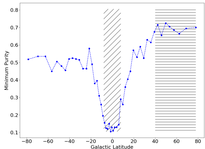
Fig. 18. The minimum purity of the published alert stream as a function of Galactic latitude (see text for details). The behaviour as a function of Galactic latitude may be understood by considering the coverage of other transient surveys which generally avoid the plane, are not full sky and are biased towards northern skies (ASAS-SN is the only other all sky transient survey). Additionally, very few alerts towards the Galactic plane are followed up. The hatched regions show ranges in Galactic latitudes which are used in the purity analysis (Sections 4.1.1 and 4.1.3). The horizontal hatched region contains 1661 published alerts and has an overall minimum purity of 0.69. The diagonal hatched region covering \pm 8 degrees around the Galactic plane contains 1628 published alerts and has an overall minimum purity of 0.09.
