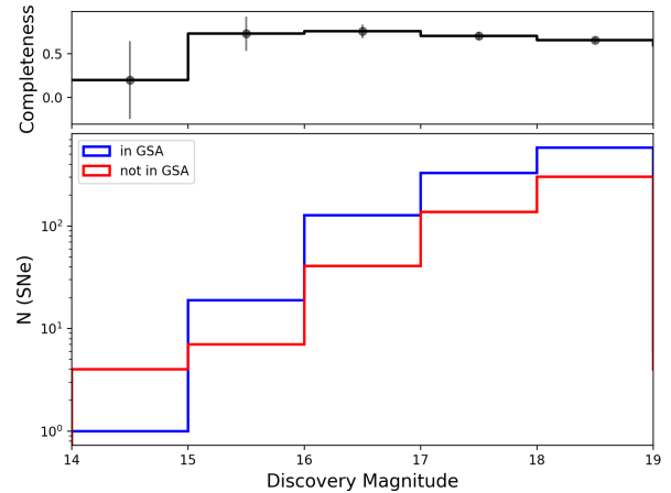
Fig. 22. Completeness as a function of magnitude for SNe with 2 or more Gaia scans. Main panel: histograms are divided into two samples: blue independently detected and published by GSA , red not detected and published by GSA . Upper panel: fraction of the total number detected by GSA .
