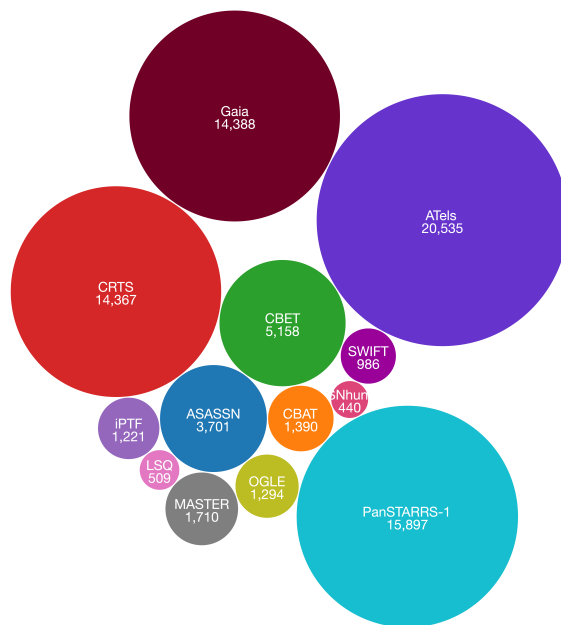
Fig. 8. Circles are proportional in area to the unique numbers of objects/events (also shown in text), compiled for the GSA database, and colour-coded by the data source. The circle for Gaia is shown for comparison. References for the surveys are given in the text. The data are taken from a snapshot of our archive on 24 November 2020.
