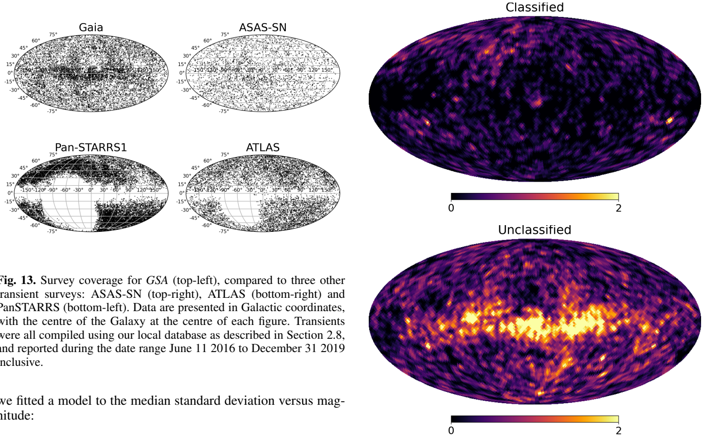
Fig. 14. Distribution on the sky for classified (upper panel) and unclassified (lower panel) alerts. The map is in Galactic coordinates, using a HEALpix grid with a resolution of about 1.8 degrees (level 5, NSIDE=32, 12288 pixels), and has been lightly smoothed.
