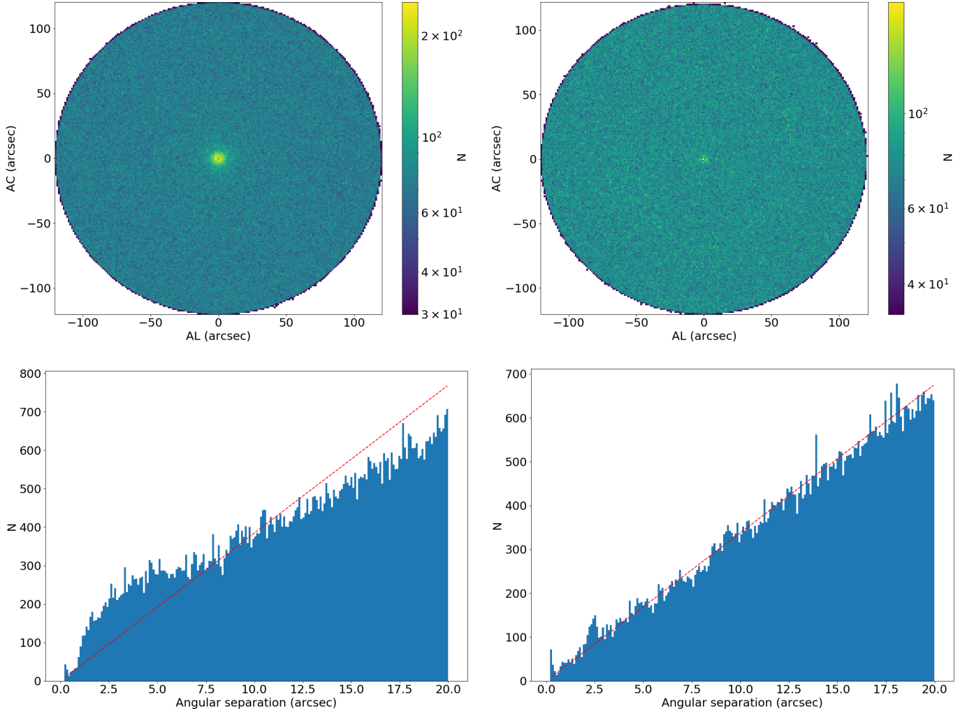
Fig. 20. Top: The number of neighbouring sources within 2' of each published alert in the AL and AC directions at the time of the alert, accumulated for all NewSource alerts (Left), and for all OldSource alerts (Right). Again all sources within 0.2'' of the alert positions are excluded as they are deemed to belong to the alerts themselves. Bottom: The number of neighbouring sources as a function of angular separation out to 20'' around the published alert, accumulated for all NewSource alerts (Left), and for all OldSource alerts (Right). The red dashed line is the expectation for the number of sources based on the assumption of the same number of sources per unit area. Here we can see that the excess in the number of sources at very close angular separations, is much more pronounced for NewSource alerts than for OldSource alerts. The range of angular separations in which there is an excess in the number of neighbouring source is more clearly seen in the bottom panels. A small excess is still visible around 2.5'' for OldSource alerts.
