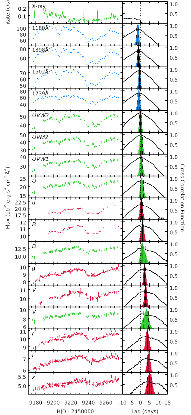
Figure 12. Left: Mrk 817 continuum light curves from HST (blue), Swift (green) and ground-based telescopes (red). All fluxes have units of 10^{-15} erg \text{s}^{-1} \text{cm}^{-2} \text{\AA}^{-1} , aside from the Swift 0.3 – 10 keV X-ray light curve which is shown as a count rate. Right: Solid black lines show the cross-correlation function with respect to the Swift UVW2 band. Colored histograms show the ICCF centroid lag distributions, while the vertical solid and dashed lines give the lag and 1\sigma uncertainty range.
