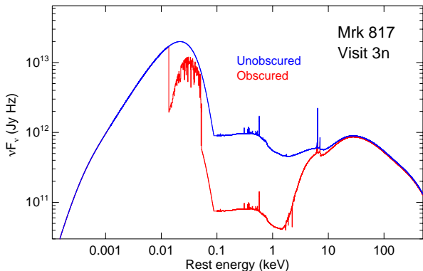
Figure 8. SED model of Mrk 817, before and after adding absorption by the obscuring gas. The unobscured SED (blue) has a luminosity of 1.1 \times 10^{45} erg s ^{-1} ( L/L_{\text{Edd}} = 22\% ), and the obscured (red) has 6.7 \times 10^{44} erg s ^{-1} .
