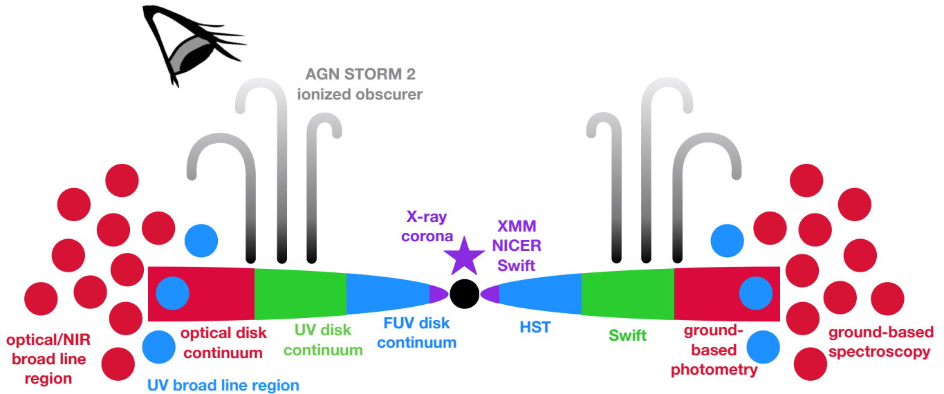
Figure 1. Schematic overview of the AGN STORM 2 campaign, highlighting the telescopes involved thus far, and what regions they probe. The color schemes correspond to different telescopes/wavelength regimes, and will be used throughout this paper and future papers. The most unexpected result is the presence of a new dust-free ionized wind, as evidenced by the presence of new narrow and broad UV absorption lines (Fig 2), and a significant depression of soft X-rays relative to earlier observations (Fig. 3). Spectral decomposition (Section 3.1.1, Section 3.1.2) and photoionization modelling (Section 3.3) place the new absorber at the inner broad line region. Despite this unexpected wind, the optical/UV continuum reverberation lags appear to behave as expected for reprocessing in a standard thin disk (Section 3.4.1 and Fig. 13). The broad line region reverberation is more complex, as the H\beta lags behave as expected, but the UV broad emission lines are uncorrelated with the continuum for the first \sim 60 days, likely due to interference from the obscurer (Section 3.4.2 and Fig. 14).
