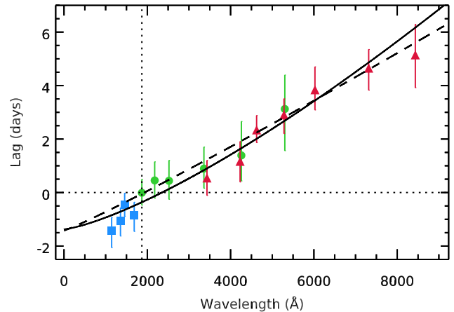
Figure 13. Continuum lags (rest-frame) calculated with respect to the Swift /UVW2 band. Data from HST , Swift and ground-based telescopes are shown as blue squares, green circles, and red triangles respectively. The solid line shows the best-fitting \tau \propto \lambda^{4/3} relation. The dashed line is the best-fitting model using the relations in Kammoun et al. (2021a), with a maximal black hole spin.
