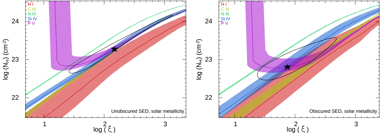
Figure 11. \log N_{\text{H}} vs \log \xi for the unobscured ( left ) and obscured ( right ) SED models. The ions in the outflow system, represented by the colored bands, provide constraints on N_{\text{H}} and \xi in the form of upper and lower limits, as well as measurement values, of measured column densities. Dotted lines are upper limits, dashed lines are lower limits, and solid lines are measurements. The uncertainty in the column density measurements are represented by the shaded bands. The solution found with \chi^2 minimization is represented by the black star, and the 1\sigma is represented by a black ellipse.
