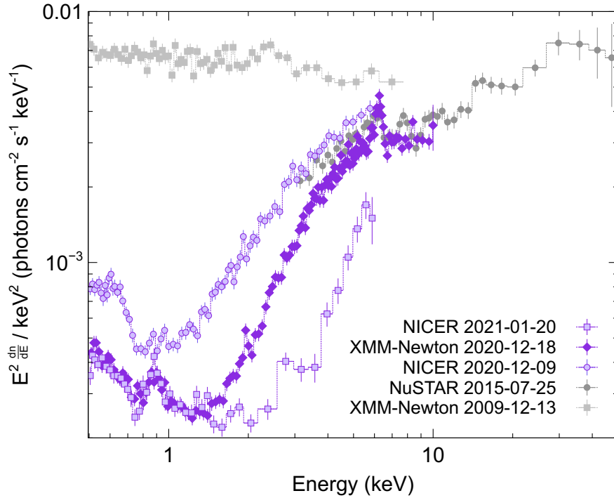
Figure 3. X-ray counts multiplied by an E^2 powerlaw, illustrating the change in spectral shape between earlier observations from XMM-Newton in 2009 and NuSTAR in 2015 (gray), and the new observations (XMM-Newton in purple diamonds and NICER in lighter purple circles).
