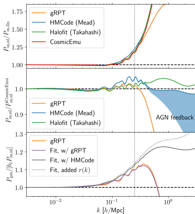
Fig. 1. Comparison of 3D power spectra, computed at z = 0.38 and the parameters listed in Table A.1. Top: Non-linear matter power spectra relative to the linear matter power spectrum, for the gRPT perturbative model, the Mead et al. (2015) HMCode, the Takahashi et al. (2012) Halofit prescription, and the CosmicEmu emulated power spectrum (Heitmann et al. 2014). Centre: Non-linear matter power spectra relative to the CosmicEmu model. The blue shaded region covers the power spectrum range within the prior range of our AGN feedback description. Bottom: Full galaxy-matter power spectrum P_{gm} relative to the Mead et al. (2015) power spectrum multiplied by the linear galaxy bias, shown for the gRPT perturbation theory model (orange) and the fit formula of Eq. (3), using gRPT (purple) or Mead et al. (2015) (grey) for the non-linear matter power spectrum term. The dotted grey curve includes an additional r(k) term obtained from a semi-analytic model of a galaxy sample similar to the one used in our analysis. The vertical grey line indicates the smallest scales used in the galaxy clustering modelling.
