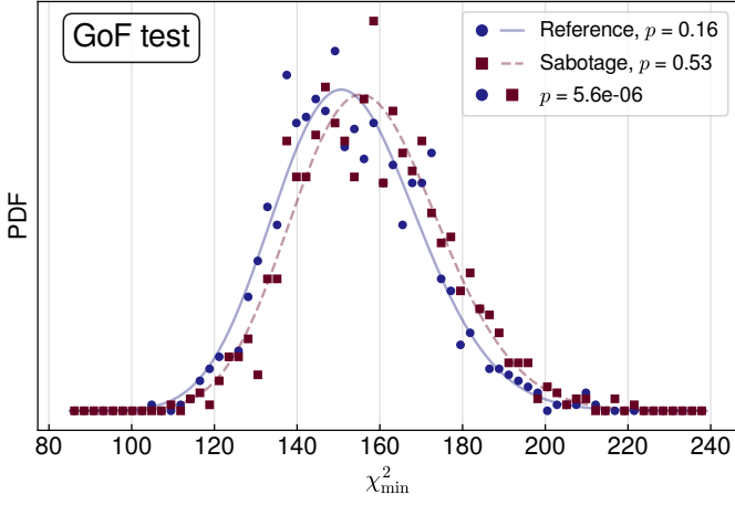
Fig. 18. Goodness of fit sampling distributions. Shown are histograms of minimum \chi^2 -values obtained from 1000 mock realisations of data vectors analysed with our cosmic shear and GGL analysis pipeline. Blue points correspond to our baseline setup; red points to the result using a sabotaged data vector computed with the S3 and S4 redshift distributions systematically shifted upwards by 5\sigma of their Gaussian prior width. The curves are best fits of a \chi^2 -distribution with its mean as free parameter. The solid blue curve is a good fit to the baseline results ( p -value of 0.16), while the sabotaged distribution is still well fitted by a \chi^2 -distribution (red dashed curve; p = 0.53 ) which however is incompatible with the baseline ( p < 10^{-5} ).
