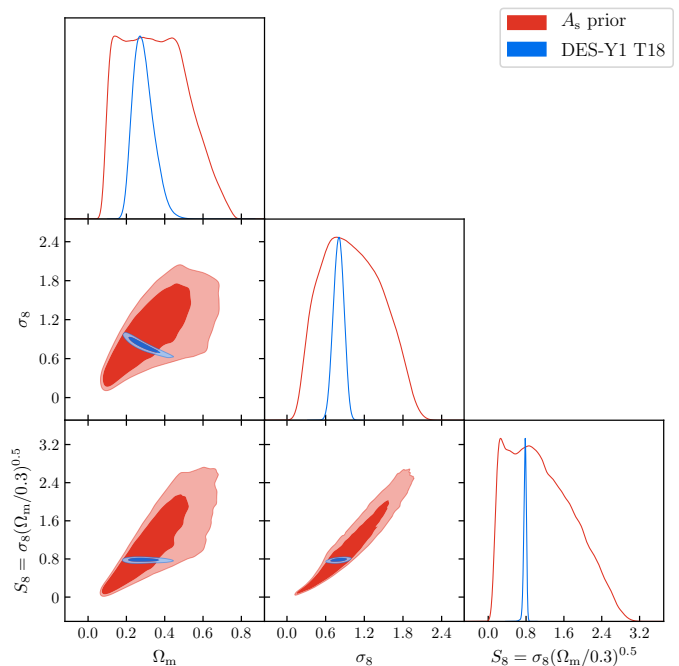
Fig. 16. Same as Fig. 15, but now showing the prior volume using the sampling parameter A_s with a wide top-hat prior, alongside the DES Year 1 cosmic shear posterior. Note the smaller axis range for the \sigma_8 and S_8 parameters compared to Fig. 15.
