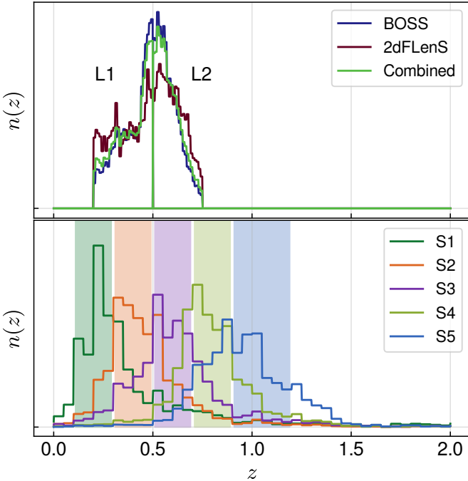
Fig. 6. Redshift distributions of the lens (upper panel) and source (lower panel) galaxy samples. Lens galaxies are split at z = 0.5 into two redshift bins for both the BOSS and 2dFLenS surveys. Modelling is carried out with a weighted combination of their redshift distributions (in green). Lens distributions are constructed for galaxies in the KiDS overlap regions, respectively. Source galaxies are split into five tomographic bins based on their best photometric redshift estimates, as indicated by the shaded bands. The source redshift distributions are KiDS-1000-like and built from KV450 data.
