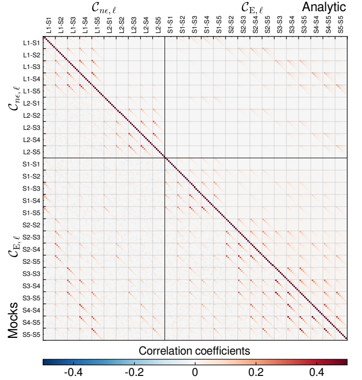
Fig. 14. Comparison of correlation coefficients of the weak lensing band power covariance between mocks (lower left) and analytic covariance (upper right) in the most realistic setup (Egretta). The top left block is for GGL; the bottom right block for cosmic shear. Galaxy sample combinations are indicated on the axes.
