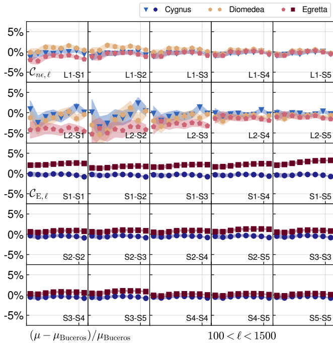
Fig. 9. Comparison of mean estimates of band power between different mock setups. Plotted is the relative deviation from the Buceros case (rectangular mask, uniform depth). Blue, yellow, and red colours correspond to the Cygnus (realistic mask, uniform depth), Diomedea (like Cygnus but using individual lens sample properties for BOSS and 2dFlenS, hence only shown for GGL), and Egretta (realistic mask and depth variations) cases, respectively. The top two rows show GGL signals; the bottom three the cosmic shear signals, with bin combinations indicated in the panels (those not used in the likelihood analysis are greyed out). Bands around the data points indicate the standard error determined from a jackknife estimate of variance on the ratios shown, based on mean signals calculated from 1000 realisations.
