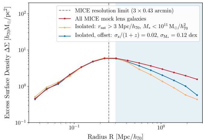
Fig. A.3. Simulated ESD profile of the offset isolated MICE sample (blue line), created by using MICE galaxies with randomly offset redshifts ( \sigma_z/[1+z] = 0.02 ) and stellar masses ( \sigma_{M_*} = 0.12 dex) when selecting the isolated lenses. This is done in order to mimic the effect of the KiDS-bright measurement uncertainties on the isolation criterion. Compared to the ESD profile of the truly isolated MICE sample (orange line) the offset sample has a \sim 30\% higher signal at large scales due to the contribution of satellites. We therefore take extra care with KiDS-bright results at R > 0.3 h_{70}^{-1} Mpc (light blue shaded region). Nevertheless, the ESD of the offset isolated MICE sample is significantly lower than that of all MICE galaxies (red line), created without any isolation criterion. In addition, we show the radius corresponding to three times the resolution of the MICE simulation (dashed vertical line), which in the case of the isolated MICE sample is R < 0.25 h_{70}^{-1} Mpc. Throughout this work, we only use the MICE results beyond this radius.
