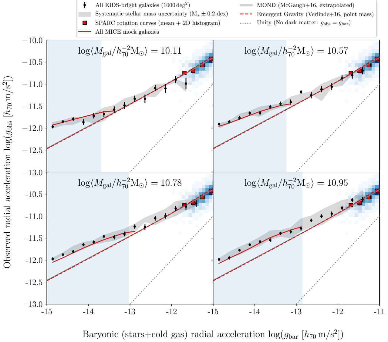
Fig. A.4. Measured RAR of all GL-KiDS lenses (black points with 1\sigma error bars) divided into four stellar mass bins, with the mean galaxy mass (stars+cold gas) of the lenses shown at the top of each panel. This figure primarily shows the effect on the RAR when the isolation criterion is not applied, which is quite significant and depends on the stellar mass of the galaxies (which correlates with galaxy clustering). The extrapolated M16 and EG predictions (grey solid and red dashed lines) function merely as a reference, showing the approximate location of the isolated galaxy RAR. They do not represent predictions in this case because g_{\text{bar}} is calculated using only the baryonic masses of the main lens galaxies (without including the baryonic masses of the satellites). The predictions from the MICE simulation (red line) match with our observations, which shows that the clustering simulated within MICE, driving the low-acceleration upturn due to the two-halo term, is indeed quite accurate.
