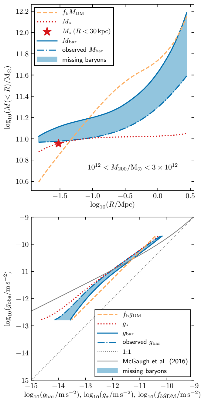
Fig. 1. Mass profiles and RAR of BAHAMAS galaxies. Upper panel: Cumulative mass profiles of stars (red dotted line) and total baryons (blue solid line) for BAHAMAS galaxies with 1 < M_{200}/(10^{12} h_{70}^{-2} M_{\odot}) < 3 . The star marker indicates the stellar mass within a 30 h_{70}^{-1} \text{kpc} aperture, indicative of what is typically regarded as the stellar mass of a galaxy. The blue dash-dotted line shows the typical baryonic mass profile of observed galaxies of similar mass, estimated based on an extrapolation of the compilation in fig. 7 of Tumlinson et al. (2017). In the inner galaxy the discrepancy (light blue shaded region) between the observed and simulated M_{\text{bar}} is relatively small, but in the outer galaxy the majority of the baryons predicted to be present in BAHAMAS consist of currently unobserved, missing baryons. The orange dashed line shows the expected baryonic mass profile if the baryon density is everywhere equal to a fixed fraction f_b = \Omega_b/\Omega_m of the local DM density. At large enough radii ( \gtrsim 2 h_{70}^{-1} \text{Mpc} ), the baryon-to-DM ratio converges to the cosmic average. Lower panel: As in upper panel, but in acceleration space. The cosmic baryon fraction provides a strong theoretical upper limit on g_{\text{bar}} at low accelerations in the context of the \Lambda\text{CDM} cosmology.
