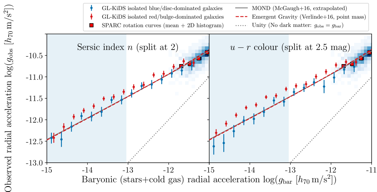
Fig. 8. Measured RAR of the KiDS-bright isolated lenses (points with 1\sigma error bars) divided into canonically early- and late-type galaxies. In the left panel, the lenses are split by Sérsic index ( n \geq 2 ) into bulge-dominated (red points) and disc-dominated (blue points) galaxies. In the right panel they are split by u - r colour ( m_u - m_r \geq 2.5 ) into red and blue galaxies (with correspondingly coloured points). In both panels we find a significant difference between the RAR measurements of early and late galaxy types. The extrapolated MOND and EG predictions (grey solid and red dashed lines) and the SPARC data (red squares with 2D histogram) are shown as a reference.
