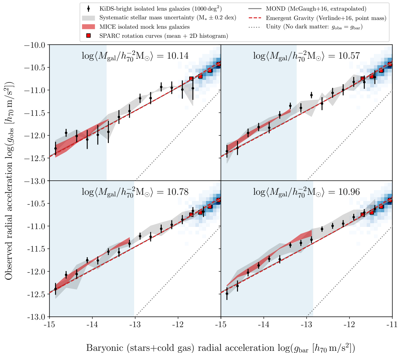
Fig. 9. Measured RAR of isolated KiDS-bright lenses (black points with 1\sigma error bars) divided into four stellar mass bins. The mean galaxy mass (stars+cold gas) of the lenses is shown at the top of each panel. At increasing stellar mass, the measurements seem to rise above the predictions from MOND (grey solid line) and EG (red dashed line). However, at scales larger than R > 0.3 h_{70}^{-1} \text{Mpc} (light blue shaded region) this could be caused by false positives in the isolated galaxy sample due to the KiDS-bright redshift uncertainty.
