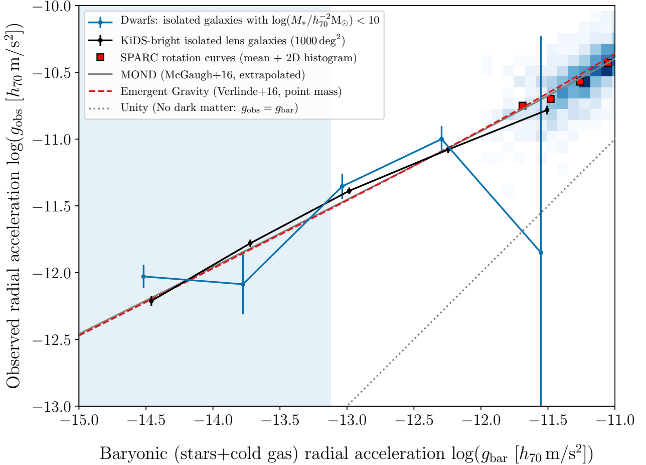
Fig. 10. Measured RAR of KiDS-bright lenses (points with 1\sigma error bars), respectively for isolated dwarfs ( \log(M_*/h_{70}^{-2}M_\odot) < 10 , blue) and the full isolated galaxy sample ( \log(M_*/h_{70}^{-2}M_\odot) < 11 , black). Due to the low S/N ratio of the dwarf lensing signal, the number of g_{\text{bar}} -bins is reduced from 15 to 5. We find that the RAR of dwarfs is consistent with that of our regular sample, and with the extrapolated MOND and EG predictions (grey solid and red dashed lines), which are shown as a reference.
