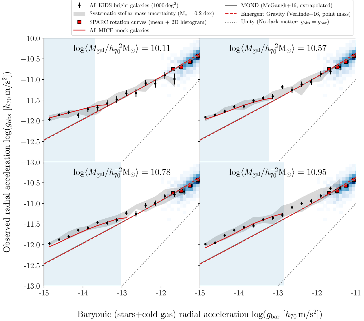
Fig. A.4. Measured RAR of all GL-KiDS lenses (black points with 1σ error bars) divided into four stellar mass bins, with the mean galaxy mass (stars+cold gas) of the lenses shown at the top of each panel. This figure primarily shows the effect on the RAR when the isolation criterion is not applied, which is quite significant and depends on the stellar mass of the galaxies (which correlates with galaxy clustering). The extrapolated M16 and EG predictions (grey solid and red dashed lines) function merely as a reference, showing the approximate location of the isolated galaxy RAR. They do not represent predictions in this case because g_{\text{bar}} is calculated using only the baryonic masses of the main lens galaxies (without including the baryonic masses of the satellites). The predictions from the MICE simulation (red line) match with our observations, which shows that the clustering simulated within MICE, driving the low-acceleration upturn due to the two-halo term, is indeed quite accurate.
