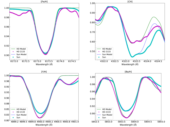
Fig. 10. Spectral synthesis of features used to derive the values of [\text{Fe}/\text{H}] , [\text{C}/\text{H}] , [\text{Y}/\text{H}] , and [\text{Ba}/\text{H}] for HD 2133, and a comparison with the solar spectrum broadened to \text{FWHM} = 25 \text{ km s}^{-1} . It is important to notice that the x-scale is the same as in Fig. 9.
