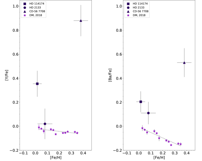
Fig. 12. Y (left) and Ba (right) abundances as a function of metallicity [Fe/H] for our three Solar-type stars with WD companions (black symbols with error bars), compared to abundances for normal Solar-type stars determined by Delgado Mena et al. (2018).
