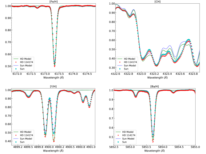
Fig. 9. Spectral synthesis of features used to derive the values of [\text{Fe}/\text{H}] , [\text{C}/\text{H}] , [\text{Y}/\text{H}] , and [\text{Ba}/\text{H}] for HD 114174, and a comparison with the solar spectrum.
