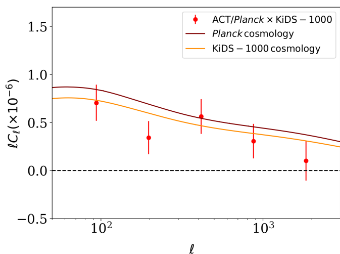
Fig. 5. The theoretical cross correlation power spectrum assuming a Planck or KiDS-1000 cosmology, compared to the combined-survey results estimated by inverse-variance weighting the ACT×KiDS-N and Planck ×KiDS-S (shown here in red).
