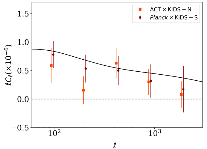
Fig. 2. The Planck best-fit model, from primary CMB anisotropies, of the cross-correlation E-mode is plotted as the solid black line. We detect non-zero correlation power at 3.1\sigma/4.3\sigma significance for ACT/ Planck ×KiDS respectively.
