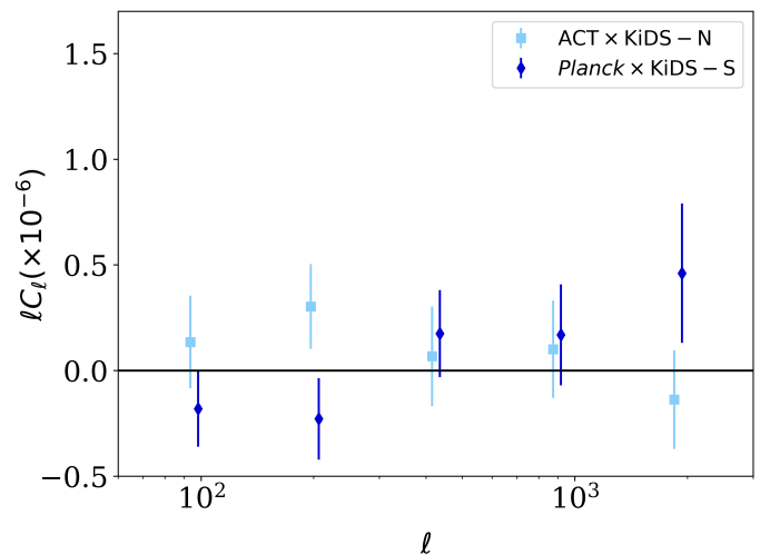
Fig. 3. The B-mode null tests, C_{\ell}^{\text{KC}\gamma\text{B}} , are consistent with zero with a p -value of 0.8/0.9 respectively using the full covariance.
