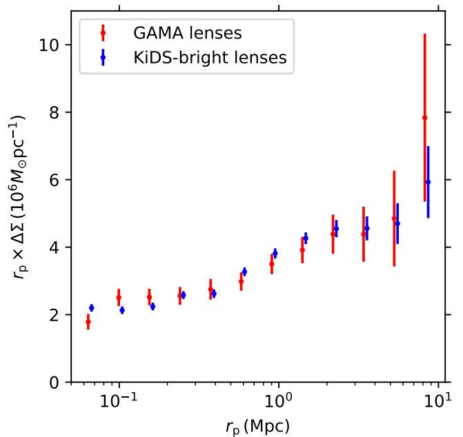
Fig. 7. Stacked excess surface density profiles, \Delta\Sigma (multiplied by the distance from the lens r_p in Mpc), around lenses with \log(M_\star/M_\odot) \in [10.5, 11.0] . The red points show results for 68 000 lenses selected from GAMA, whereas the blue points show the signal around 352 000 lenses from the KiDS-Bright sample. The KiDS measurements are shifted slightly to the right for clarity.
