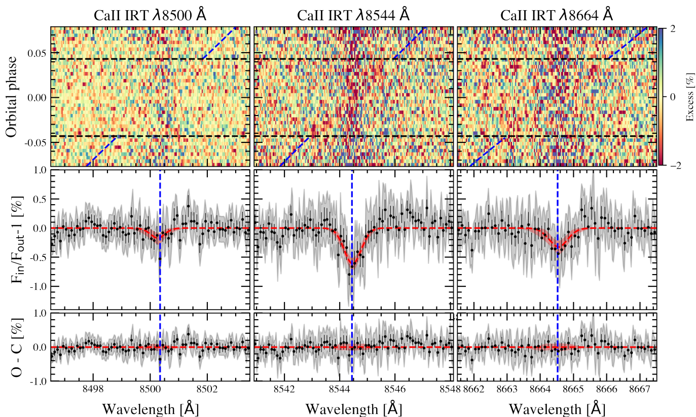
Fig. 8: Transmission spectra obtained around the three lines of the Ca II IRT triplet, as a result of combining the two nights. Top panels : tomography maps shown in the stellar rest frame. The orbital phase of the planet is presented in the vertical axis, the wavelength (in vacuum) in the horizontal axis, and the flux excess information is shown in the colour bar (in %). The data are shown binned by 0.004 in orbital phase. The tilted blue-dashed lines show the position of the spectral lines in the planet rest frame. The black-dashed lines show the first and last contact of the transit ( \phi = \pm 0.043 ; Ehrenreich et al. 2020). Middle panels : transmission spectra computed considering the data between the first and last contacts of the transit. In light grey we show the uncertainties of the original data sampling, and in black the data binned by 0.1 Å. The blue-dashed lines show the laboratory wavelengths of the lines, the red-dashed line the best-fit Gaussian profile, and the light red regions indicate the 1\sigma uncertainties of the profiles. Bottom panels : Residuals between the observed transmission spectra and the best-fit Gaussian profiles shown in the middle panel.
