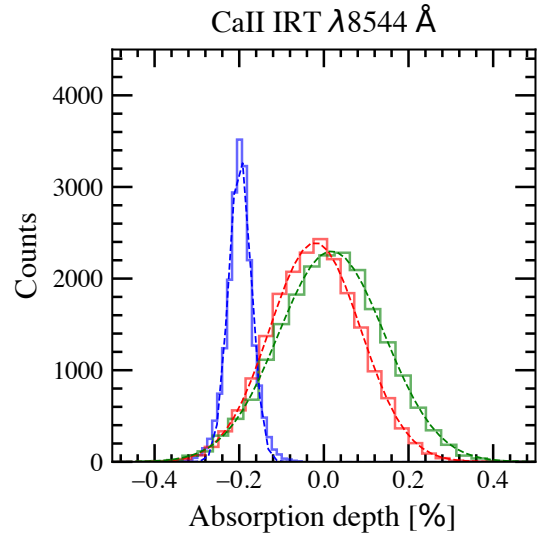
Fig. 15: EMC distributions around the Ca II IRT 8544 \text{ \AA} line for both nights combined. The results of the ‘in-in’ sample are shown in red, the ‘out-out’ in green, and the ‘in-out’ in blue. The dashed lines show the best-fit Gaussian profiles of the distributions.
