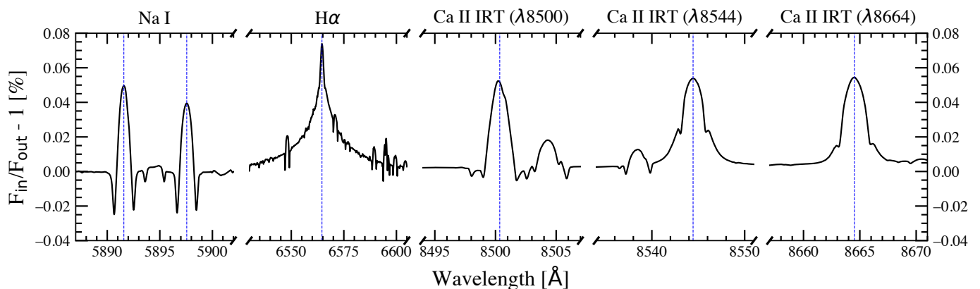
Fig. 4: Modelled RM and CLV effects on the transmission spectrum of WASP-76b around some of the spectral lines studied here: Na I doublet, H\alpha , and Ca II IRT lines. These effects are calculated based on the ATLAS9 stellar atmospheric models with LTE. The transmission spectra are calculated in the planet rest frame. The vertical blue-dashed lines show the laboratory position of the spectral lines in vacuum.
