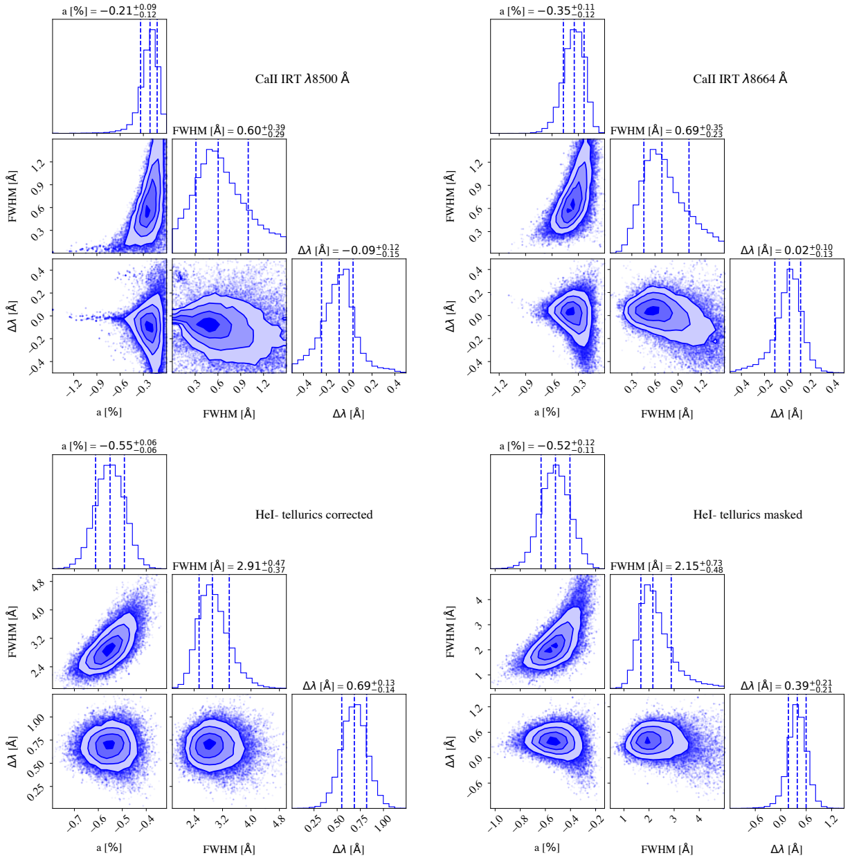
Fig. A.5: MCMC probability distribution of the Gaussian profile parameters for the Ca II IRT \lambda 8500 Å and \lambda 8664 Å ( top row ), and the He I \lambda 10830 Å (corrected and masked tellurics, bottom row ) absorption lines observed in the transmission spectrum of WASP-76b. The distributions were obtained using 10^4 steps and 10 walkers.
