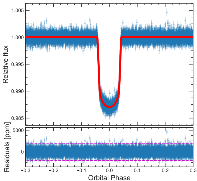
Fig. 7: Top panel : TESS phase-folded light curve centered on the transit of WASP-76b. The red line shows the best-fit transit model. Bottom panel : residuals between the phase-folded light curve and the best-fit model. The magenta dashed lines depict the residual standard deviation multiplied by three, which points to no significant anomalies inside the transits in comparison to the points out of transit.
