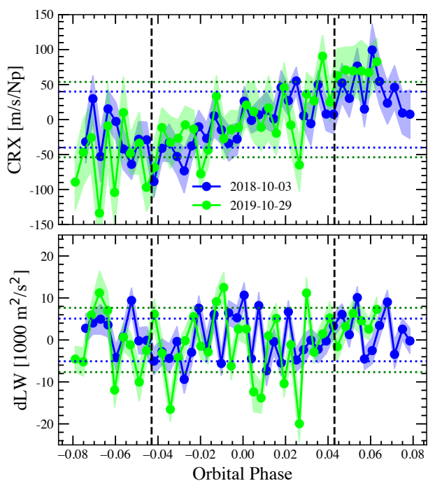
Fig. 5: Activity indices derived with serval for the two observing nights, shown in blue and green lines, respectively. Top panel : chromatic radial-velocity index (CRX). Bottom panel : differential line width (dLW). The horizontal dotted lines show the standard deviation of the values for the first (blue) and second night (green).
