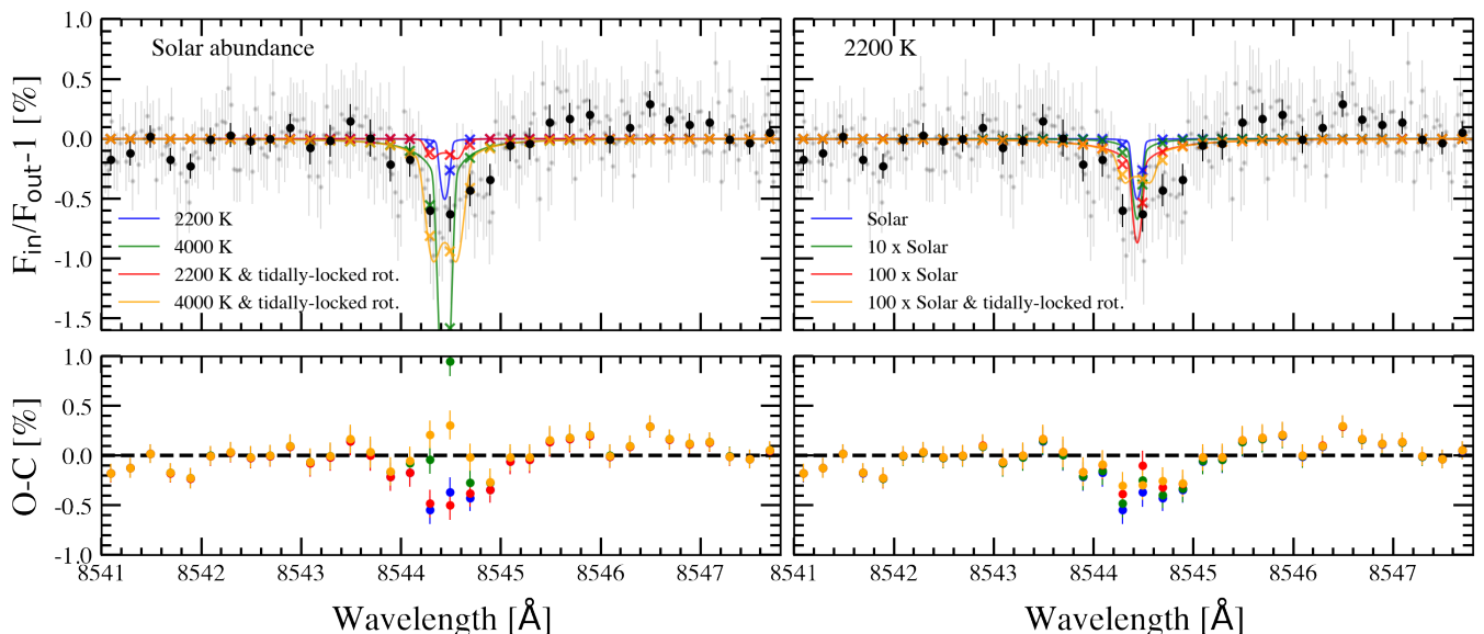
Fig. 10: CARMENES transmission spectrum of WASP-76b obtained around the Ca II IRT \lambda 8544 \text{ \AA} line compared to different atmospheric models. Top panels: The original data are shown in light grey, the data binned by 0.2 \text{ \AA} are shown in black dots, and the models binned by the same amount are presented in coloured crosses. Top left panel: models computed assuming solar abundance. The blue and green lines show the transmission models derived assuming 2200 K and 4000 K, without considering rotational broadening. In red and orange we present the atmospheric models at these same temperatures, but considering a tidally locked rotational broadening. Top right panel: atmospheric models computed assuming a temperature of 2200 K but considering different abundances: solar (blue; same as in the top panel), 10 times solar (green), 100 times the solar abundance without (red) and with (orange) tidally locked rotation. Bottom panels: residuals between the transmission spectrum and the different models (same colours as in top panels). The black-dashed line shows the reference at 0%.
