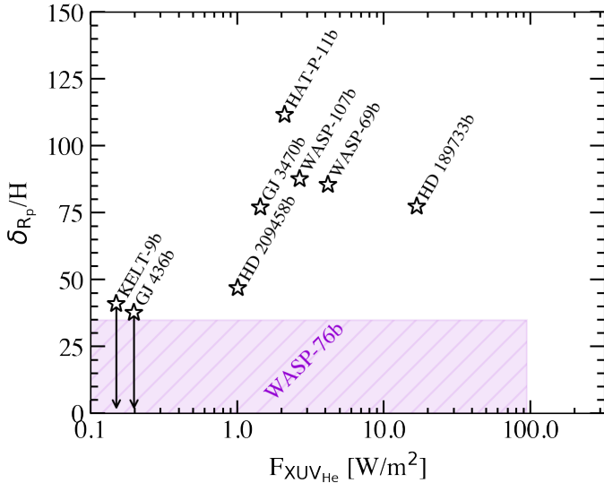
Fig. 14: He I transmission signals measured using observations at high spectral resolution with CARMENES, as a function of the XUV He flux ( \lambda < 504 \text{ \AA} ) received by the planet. The vertical axis shows the equivalent height of the He I atmosphere \delta_{R_p} , normalised by its atmospheric scale height in the lower atmosphere, H , calculated assuming \mu = 2.3 and the equilibrium temperature of the planets. The coloured region shows the constrained ranges defined by the He I absorption and XUV He flux upper limits measured for WASP-76b. The information on the other exoplanets is extracted from Nortmann et al. (2018), Alonso-Floriano et al. (2019), and Palte et al. (2020a). The black arrows show upper limits on the measured He I absorption of KELT-9b and GJ 436 b.
