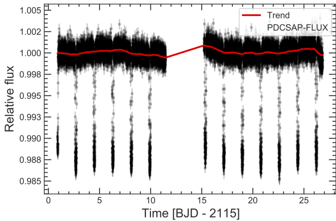
Fig. 6: TESS light curve (PDCSAP flux) of WASP-76 as observed during sector 30. The red line shows the trend obtained by applying a bi-weight detrending filter determined with wotan .
