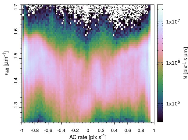
Fig. 6: Distribution in the (\mu, \nu_{\text{eff}}) plane of the observations depicted in Figure 5. There is a correlation between \mu and \nu_{\text{eff}} that evolves over time (see text).
