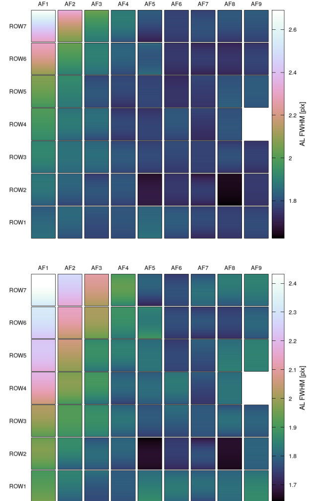
Fig. 12: Variation in the AL FWHM with AC position within each CCD and across the AF focal plane, for FOV1 (upper panel) and FOV2 (lower panel). Obtained from the calibration at revolution 3343 and for \nu_{\text{eff}} = 1.43\mu\text{m}^{-1} .
