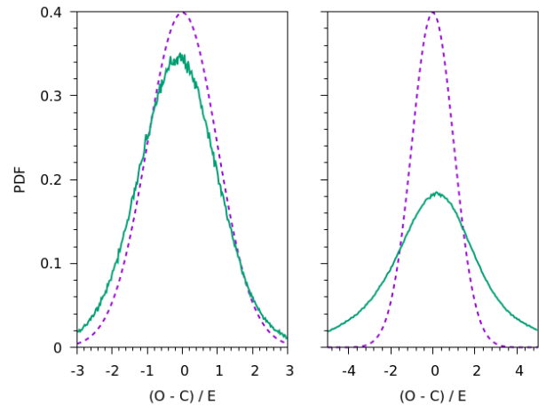
Fig. 17: Distribution of the normalised residuals about the model, for selected 1D LSF (left) and 2D PSF (right) calibrations. The data is plotted in solid green lines, and the dashed purple line shows the unit Gaussian.
