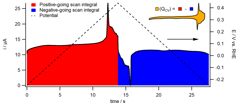
Figure C.6: Visual representation of the charges discussed in text, and what regions they represent.
