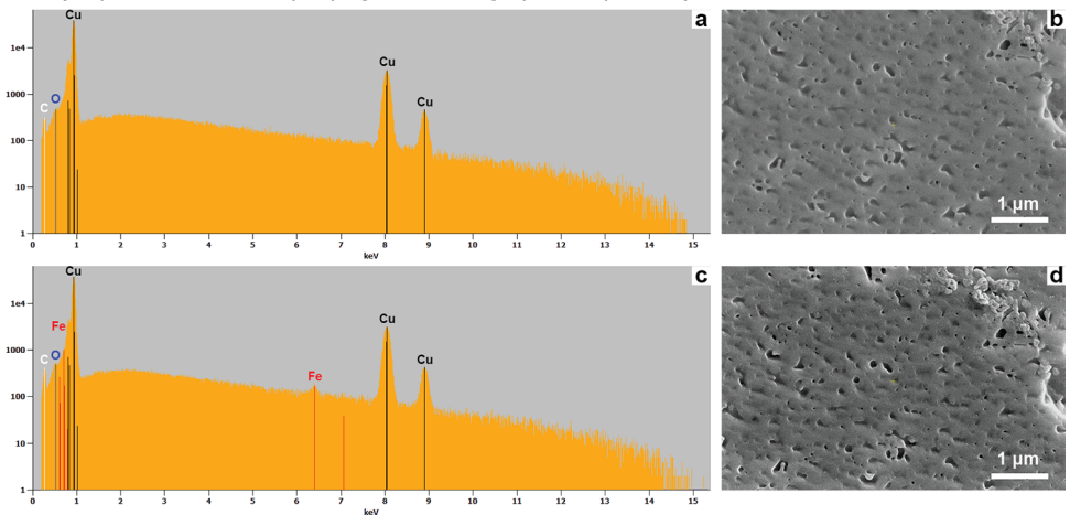
Figure D.8: Equal conditions as Figure D.7, but for a different location on the crystal. Panels a and c represent the EDX spectrum a) prior to and c) after CO2RR, whilst b) and d) represent the accompanying SEM micrographs, respectively.
