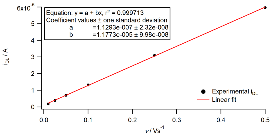
Figure C.5: Total double layer capacity ( C_{tot} ) of the polished polycrystalline copper electrode discussed in text, as calculated via Equation C.1 using experimentally determined charging currents as per Equation C.6.
