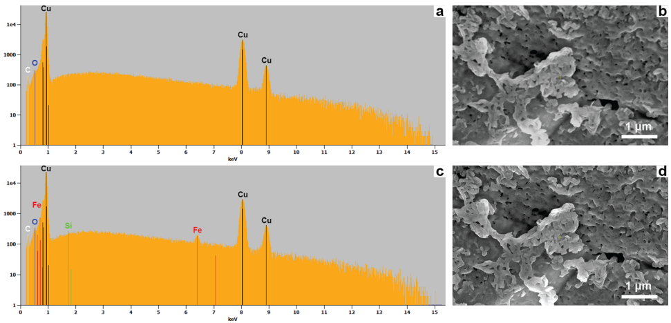
Figure D.7: Surface morphology and elemental analysis results before and after ca. 5 hours of CO2RR at -0.75 V in saturated \text{KHCO}_3 solution under constant \text{CO}_2 (g) purging for a different location than discussed in the main text with different mesoscopic morphology on a nitric acid-cleaned polycrystalline bead electrode. Panels a and c represent the EDX spectrum a) prior to and c) after CO2RR, whilst b) and d) represent the accompanying SEM micrographs, respectively.
