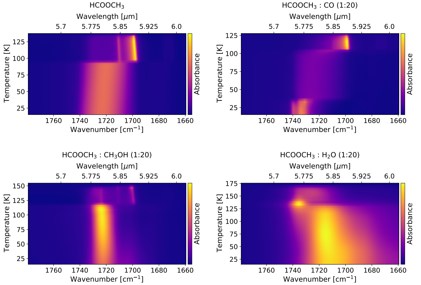
Fig. F.1. Temperature versus Spectra (TvS) heatmaps of the C=O stretching mode ( 1723.1\text{ cm}^{-1} / 5.804\text{ }\mu\text{m} ) of HCOOCH 3 in the astronomically relevant ice matrices as a function of temperature.
