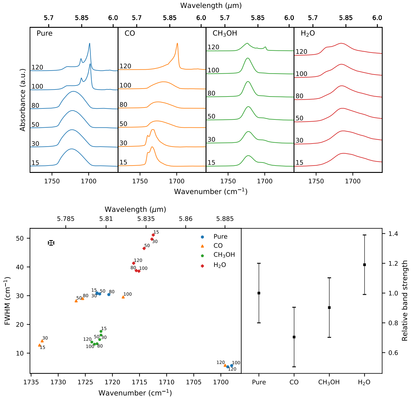
Fig. F.2. Top panel: Absorption feature of the C=O stretching vibrational mode (1723.1 cm -1 / 5.804 μm) for each of the mixtures at selected temperatures. Bottom left panel: FWHM as a function of peak position at the selected temperatures. The error bar of each individual point is given in the top left. Bottom right panel: The relative band strengths for methyl formate in the different ice matrices at 15 K with respect to the pure band strength.
