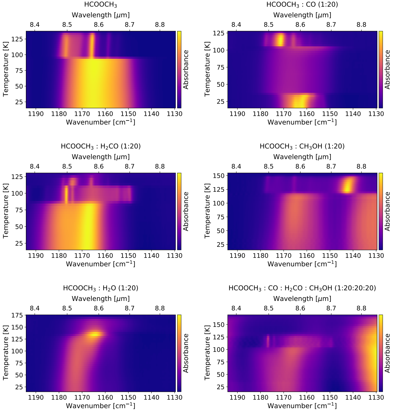
Fig. D.1. Temperature versus Spectra (TvS) heatmaps of the \text{CH}_3 rocking mode ( 1165.3 \text{ cm}^{-1} / 8.582 \mu\text{m} ) of \text{HCOOCH}_3 in the astronomically relevant ice matrices as a function of temperature.
