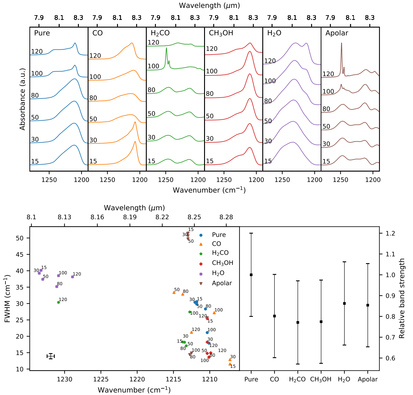
Fig. E.2. Top panel: Absorption feature of the C–O stretching vibrational mode (1211.3 cm -1 / 8.256 μm) for each of the mixtures at selected temperatures. Bottom left panel: FWHM as a function of peak position at the selected temperatures. The error bar of each individual point is given in the bottom left. Bottom right panel: The relative band strengths for methyl formate in the different ice matrices at 15 K with respect to the pure band strength.
