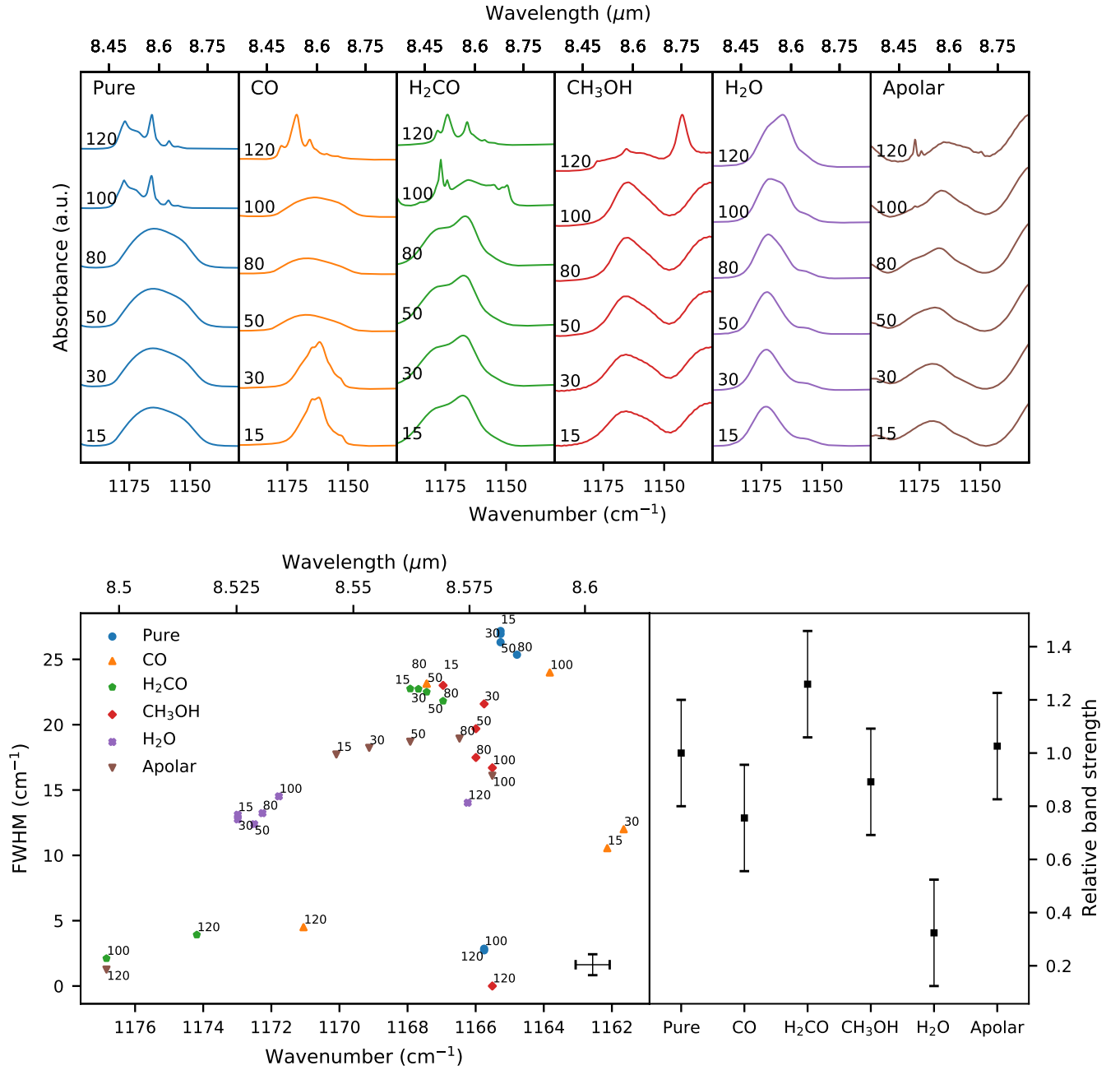
Fig. D.2. Top panel: Absorption feature of the \text{CH}_3 rocking vibrational mode ( 1165.3 \text{ cm}^{-1} / 8.582 \mu\text{m} ) for each of the mixtures at selected temperatures. Bottom left panel: FWHM as a function of peak position at the selected temperatures. The error bar of each individual point is given in the bottom right. Bottom right panel: The relative band strengths for methyl formate in the different ice matrices at 15 K with respect to the pure band strength.
