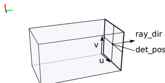
Fig. 2. Creation of typical tomographic geometries. From left to right: a volume geometry, single-axis parallel beam geometry, and a circular cone beam geometry. Below, arbitrarily oriented vector geometries are shown. The parameters are specified using keyword-only arguments [27]. The pos parameter, for instance, determines the position of a volume, other parameters have accompanying labels in the diagrams. The diagrams are created using tomosipo.
