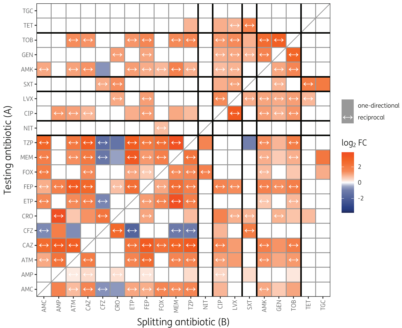
Figure 3. Heatmap of collateral responses identified based on clinical surveillance MIC data, for different antibiotic combinations. The effect size (blue/orange colour) \log_2 FC is the mean \log_2(MIC) shift between the groups low and high MIC for splitting antibiotic B. On the y-axis the tested antibiotics that were split on antibiotic B (x-axis) and the bold lines separate the different antibiotic classes. A darker colour indicates a larger effect, with orange showing CR and blue showing CS. White squares indicate no significant effect at the 0.05 FDR threshold. Reciprocity is denoted by a two-sided arrow.
