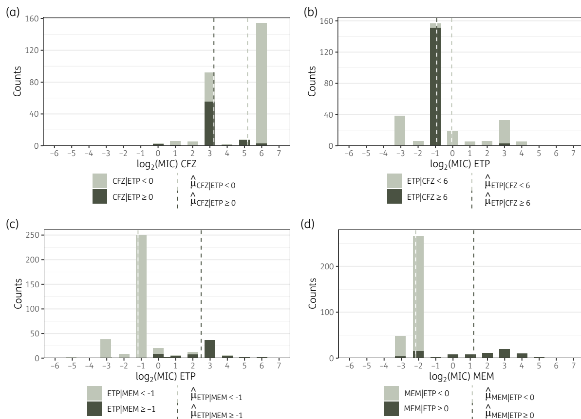
Figure 4. \log_2 transformed MIC [ \log_2(\text{MIC}) ] distributions of the most significant CS effect (a) and the most significant CR effect (c). The frequency is shown on the y-axis for the different values of the \log_2(\text{MIC}) . The different colours denote high (dark) or low (light) MIC to the splitting antibiotic. The dashed lines show the estimated means for the two groups. (a) \log_2(\text{MIC}) distribution of cefazolin (CFZ) split by MIC of ertapenem (ETP) and (b) the distribution of ertapenem under influence of cefazolin, which also has a significant CS response, showing a reciprocal effect. (c) \log_2(\text{MIC}) distribution of ertapenem under influence of meropenem, which has a significant CR response (3.66 \log_2 FC) and (d) the distribution of meropenem under influence of ertapenem, which also has a similarly sized CR response (3.37 \log_2 FC). This is a reciprocal collateral response.
