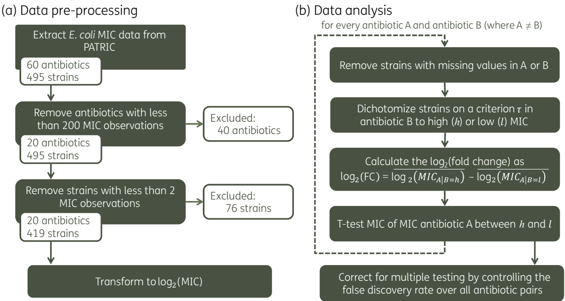
Figure 2. Data pre-processing steps (a) and data analysis strategy (b) schematic overview.
