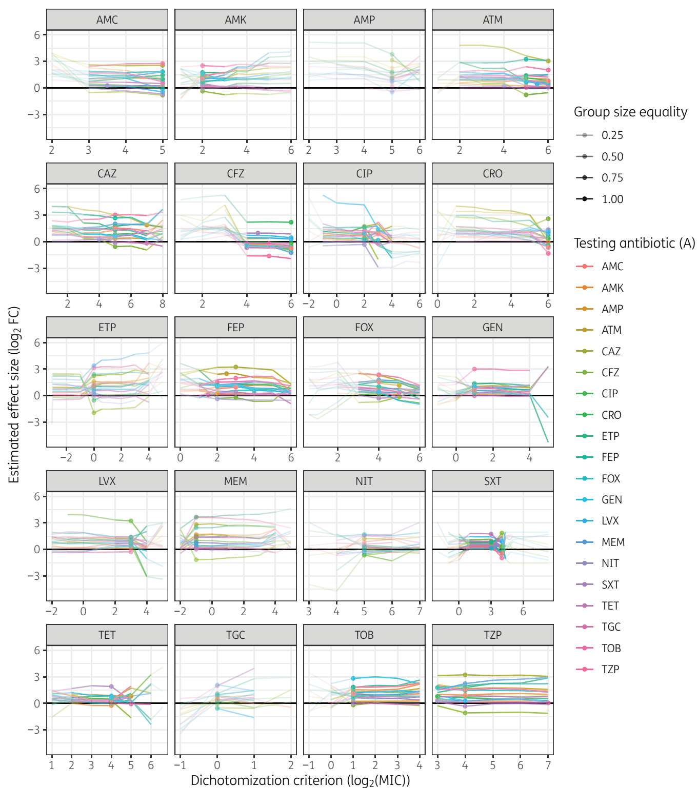
Figure 6. The effect of changing the dichotomization criterion (x-axis) on the estimated \log_2 FC (y-axis). Every panel denotes the antibiotic that is dichotomized (antibiotic B). The colours show the different antibiotics that were tested based on this dichotomization (antibiotic A). The dots denote the value of the \log_2 FC found in the main analysis, based on equal split dichotomization. A more transparent line shows a larger inequality in group sizes, where the effect estimation is driven by only a small part of the total sample. Straight horizontal lines denote stable effect size estimation over different dichotomization criteria, while crooked lines show unstable estimation.
