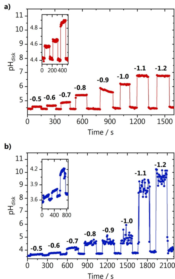
Figure 3. Interfacial pH measurement during chronoamperometry (potentials indicated in the graph in V vs. Ag/AgCl) in 0.1 M argon saturated \text{KH}_2\text{PO}_4 ( \text{pH}_{\text{bulk}} = 4.4 ) (a) and \text{K}_2\text{SO}_4 ( \text{pH}_{\text{bulk}} = 3.6 ) (b) at 1600 rpm.
