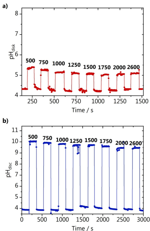
Figure 4. Interfacial pH measurements during chronopotentiometry (constant current density = -0.42 \text{ mA cm}^{-2} ) in 0.1 M argon saturated \text{KH}_2\text{PO}_4 \text{pH}_{\text{bulk}} = 4.4 (a) and \text{K}_2\text{SO}_4 \text{pH}_{\text{bulk}} = 4.0 (b) at the different rotations indicated in the graph in rpm.
