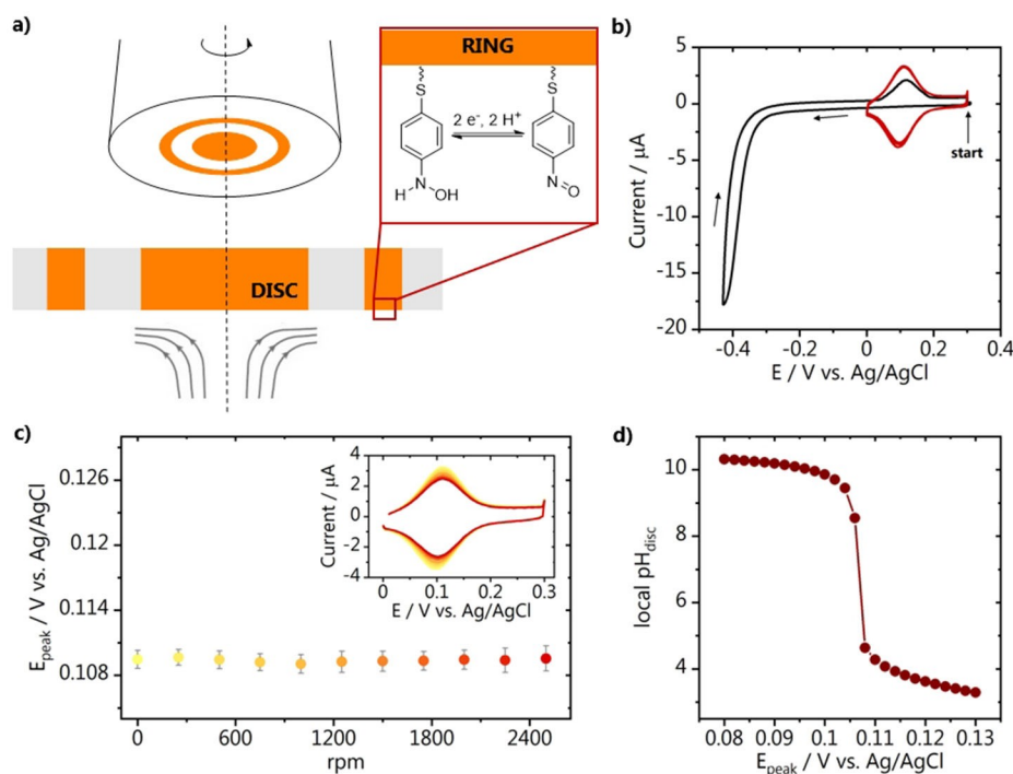
Figure 1. a) Schematic representation of the RRDE with the functionalized ring; b) cyclic voltammetry of the 4-NTP to 4-HATP conversion (black, 100 mVs -1 ) together with a characterization of the 4-HATP/4-NSTP redox couple (red, 200 mVs -1 ). Both were recorded in 0.1 M K 2 SO 4 , pH = 4. c) Effect of rotation on the pH sensor mid-peak potential, extracted from the voltammograms shown in the inset. d) Theoretical relationship between E_{\text{peak}} and \text{pH}_{\text{disc}} using Equation 7 for \text{pH}_{\infty} = 4 .
