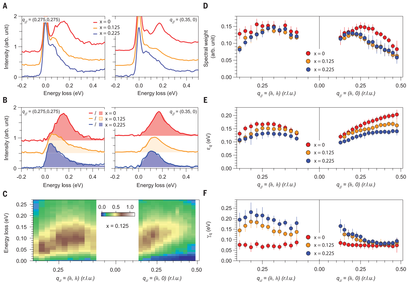
Fig. 4. RIXS spectra of \text{Nd}_{1-x}\text{Sr}_x\text{NiO}_2 . (A) Raw spectra at representative momentum positions for x = 0, 0.125 , and 0.225 at 20 K. (B) Magnetic spectra obtained by subtracting the elastic line, phonon, and background from the raw data shown in (A). The shaded areas indicate the associated DHO fitting. (C) Magnetic spectra map of \text{Nd}_{1-x}\text{Sr}_x\text{NiO}_2 ( x = 0.125 ) along hh and h directions at 20 K. (D to F) Summary of (D) spectral weight, (E) mode energy \epsilon_q , and (F)
