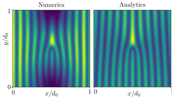
FIG. 4. Left panel: numerically calculated intensity profile |\Psi(x, y)|^2 of the zeroth Landau level in a vortex lattice with a pair of h/2e vortices at the center of the unit cell ( K = 2\Delta_0 = 40\hbar v/d_0 , \mu = 0 ). Right panel: analytical result from the solution of the Helmholtz equation (9) for a single h/e vortex [37].
