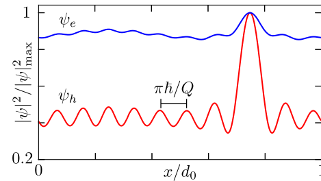
FIG. 5. Electron and hole contributions to the local density of states in the zeroth Landau level along a line parallel to the x axis which passes close to a vortex core at x = y = 3d_0/4 . The curves are plots of \sum_{\mathbf{k}} |\psi_{e,h}(x, y)|^2 normalized to unit peak height at the vortex core. The parameters are K = 2\Delta_0 = 40\hbar v/d_0 , \mu = 0.5\hbar v/d_0 . The expected oscillation period of \pi\hbar/Q = 0.091d_0 is indicated.
