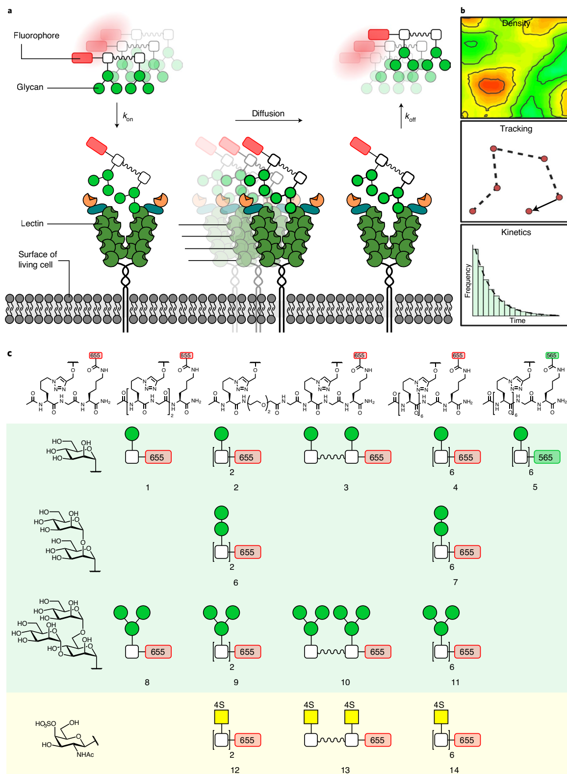
Fig. 1 | Scheme of the Glyco-PAINT procedure. a , A probe consisting of a fluorophore (depicted in red) linked to a glycan cluster (green) becomes visible when binding to the cell surface mannose receptor. b , Imaging the bound fluorescent ligand is used to determine the on-cell receptor density, tracking receptor movement, and quantify the binding kinetics of the glycans. c , The library of different mannose receptor ligands used, including ligands for the C-type lectin domains (dark green) and cysteine-rich domain (yellow) of the receptor.
