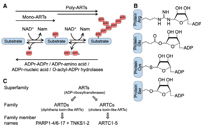
Fig. 1. ADP-ribosylation is a reversible modification of proteins, nucleic acids, and metabolites. (A) Indicated are ADP-ribosyltransferases (ARTs), which catalyze mono- and poly-ADP-ribosylation (MARylation and PARylation, respectively). Poly-ARTs may modify naïve substrates generating PAR chains. Alternatively, poly-ARTs may use MARylated substrates and extend the modification to form polymers. The modification is removed by ADP-ribosylhydrolases. Some hydrolases degrade PAR chains (e.g., PARG and ARH3), and others cleave the glycosidic bond between the substrate and the proximal ADPr (e.g., MacroD1, MacroD2, TARG1, ARH1 and ARH3). Substrates include proteins, nucleic acids, and metabolites (the latter exemplified by O-acetyl-ADPr). The specificity of the enzymes is not indicated, some are highly selective, while others have broad specificity, including the modification of different classes of substrates. (B) Indicated are proteins with different ADPr acceptor amino acids and the corresponding N-, O-, or S-glycosidic linkages at the 1' position of the nicotinamide ribose. Additional amino acids that have been detected to be modified include Asp, Asn, Lys, Thr, Tyr, His, Phospho-Ser, and diphthamide. Please note that for Ser-ADPr and Arg-ADPr, and probably for other linkages, the initial products are in the \alpha configuration. Isomerization may occur, which is indicated. Additionally, migration to the 2'- and 3'-OH may happen for Glu-ADPr and Asp-ADPr. (C) Summary of the proposed nomenclature. ARTs represent the superfamily, which consists of 23 families, two being ARTD and ARTC [17,18]. Names that are commonly used for ARTD family members are PARP (the historic abbreviation for poly(ADP-ribose)polymerase) and TNKS (for tankyrase). Here, we propose PARP as a name on its own right, rather than an abbreviation.
