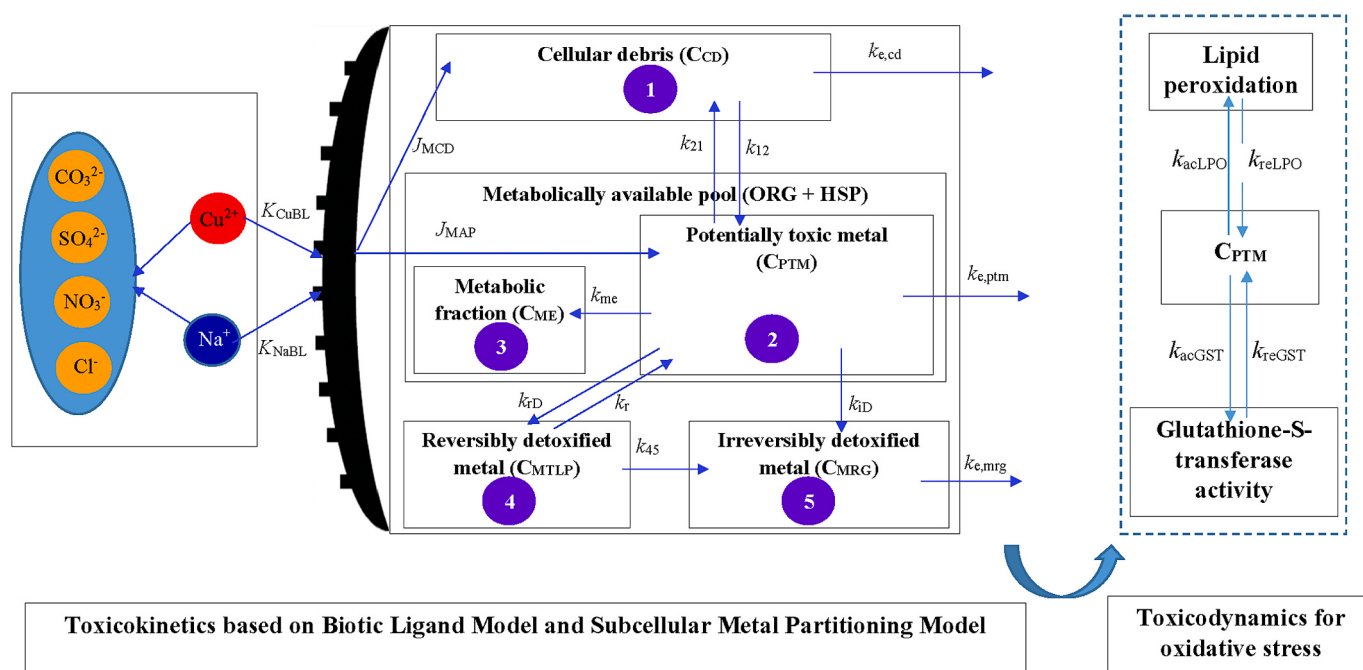
Fig. 1. A toxicokinetic-toxicodynamic (TK-TD) model with the accumulation of metals in the potentially toxic metal fraction ( \text{C}_{\text{PTM}} ) as the connecting point. Simulation of the TK phase is based on the concepts of the biotic ligand model, i.e. the metal uptake rate depends on the activity of free metal ions (speciation model) and the interactions of free metal ions with the biotic ligands at the gills (represented by the binding constants K_{\text{CuBL}} and K_{\text{NaBL}} ); and the subcellular metal partitioning model: metals taken up via gills are distributed to the metabolically available pool (including metals in association with organelles ORG and heat-sensitive proteins HSP) and the cellular debris with the rates J_{\text{MAP}} and J_{\text{CD}} , respectively. Metals can be transported between these two fractions with rates k_{12} and k_{21} . From the cellular debris, metals can be eliminated at a rate constant k_{\text{e,cd}} . Part of the metal in the MAP is used in the metabolic processes ( \text{C}_{\text{ME}} ), while the excess metal above the metabolic requirement is built-up in the potentially toxic metal pool ( \text{C}_{\text{PTM}} ) where metals can be reversibly detoxified by binding to metallothionein-like proteins with a detoxification rate constant k_{\text{TD}} ( \text{C}_{\text{MTLP}} ), irreversibly detoxified by the storage in metal-rich granules ( \text{C}_{\text{MRG}} ) with a detoxification rate constant k_{\text{ID}} , or eliminated at a rate constant k_{\text{e,ptm}} . Part of reversibly detoxified metals can be released back to the MAP, which can be used in metabolism, or internalised into the metal-rich granules with a rate constant k_{45} . Part of irreversibly detoxified metals can be eliminated at a rate constant k_{\text{e,mrg}} .
