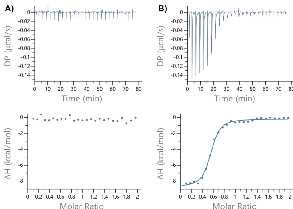
Figure 3. Titrations of LUVs containing 2 mol % lipid II and 20 mol % DOPG in DOPC (10 mM) into a solution of: (A) 20 \mu M daptomycin, 2 mM DOPG or (B) 20 \mu M nisin, 2 mM DOPG. In both cases, the buffer used consisted of 20 mM HEPES, 5 mM \text{CaCl}_2 , 150 mM NaCl, pH 7.4.
