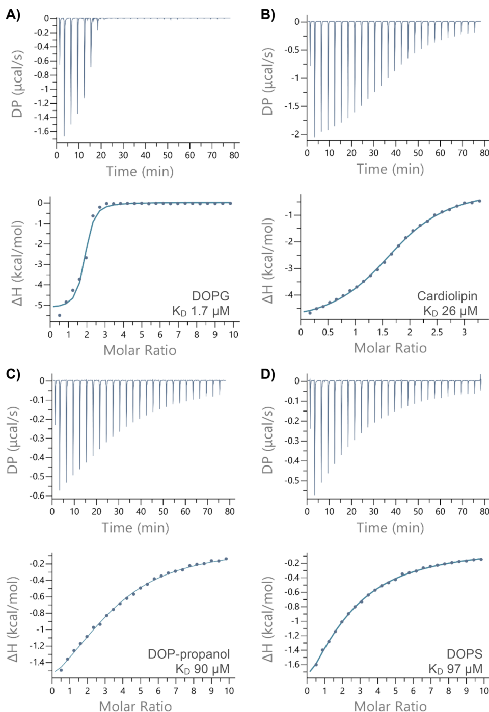
Figure 2. Representative binding isotherms for the titrations of 10 mM DOPC LUVs containing 25 mol % of: (A) DOPG (titrated into 50 \mu M daptomycin); (B) cardiolipin (titrated into 150 \mu M daptomycin); (C) DOP-propanol and (D) DOPS (both titrated into 50 \mu M daptomycin). Buffer used for all binding experiments consisted of 20 mM HEPES, 5 mM \text{CaCl}_2 , 150 mM NaCl, pH 7.4.
