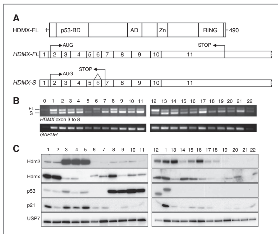
Figure 1. Analysis of HDMX-S in 22 osteosarcoma cell lines. A, schematic drawing of Hdmx protein structure (top) containing the p53-binding domain (p53-BD), acidic domain (AD), zinc-finger (Zn), and RING domain. Structure of HDMX-FL and HDMX-S mRNA is depicted below. Arrows indicate start and stop codons. Exon 6 is spliced out in HDMX-S , resulting in 26 novel amino acids and a premature stop codon. B, a total of 22 osteosarcoma cell lines and 1 osteoblast sample were examined for HDMX-FL and HDMX-S mRNA expression using primers for Hdmx exon 3 (Fw) to exon 8 (Rev). GAPDH mRNA expression was examined as an internal control. C, protein levels were analyzed with immunoblotting using the indicated antibodies. USP7 expression was analyzed as a loading control.
