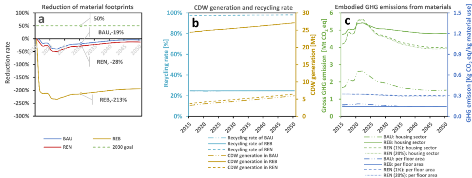
Figure 6.7 (a) Reduction rate of material footprints of three scenarios compared with 2015 level of the BAU scenario, (b) the generation of construction and demolition waste and recycling rate of three scenarios, (c) embodied GHG emissions of material uses of three scenarios. Note: The “(1%)” in (c) represents the light-weight concrete waste accounts for 1% in the gross normal-weight concrete waste from 2015 to 2050; the “(20%)” indicates the share of the light-weight concrete waste linearly increases from 1% in 2015 to 20% in 2050.
