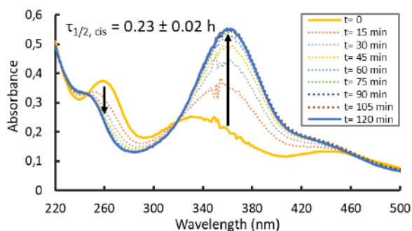
Figure S4.2: UV-Vis spectra showing the cis to trans relaxation of peptide K_{4,i,i+11} -Azo, 35 \mu M in PBS, pH 7.4. The peptide solution was irradiated with 385 nm light before relaxation was measured at a constant temperature of 25 °C. Figure adapted from the Msc. Thesis of Wessel Verbeet.
