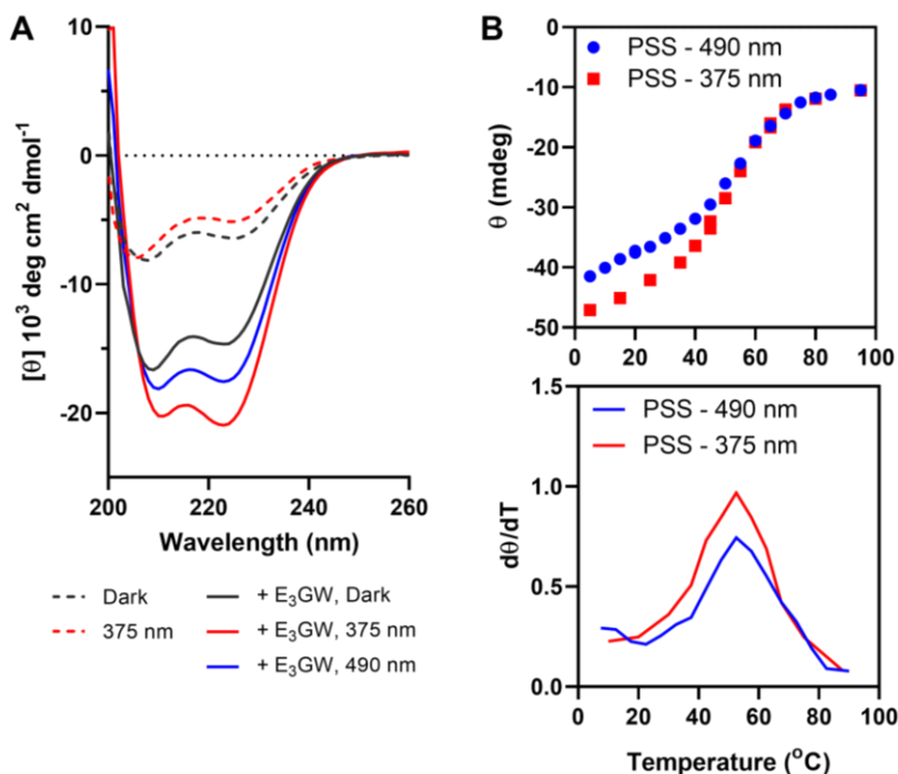
Figure 4.3: CD spectra showing the differences in folding for peptide K_3^{i,i+4} -Azo independently and as a coiled-coil with peptide E_3 GW at different photostationary states. (A) Melt curves of the coiled-coil after isomerization with either 375 nm or 490 nm light (B, top graph) and the first order derivative of these melt spectra (B, bottom graph). Spectra were recorded in PBS buffer at pH 7.4, with 50 \mu\text{M} total peptide concentration.
