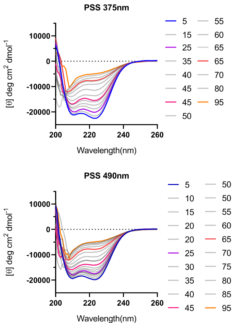
Figure S4.3: CD spectra at different temperatures (in °C) for the coiled-coil between peptide K_3^{i,i+4} -Azo and E_3 GY at 50 \mu M total peptide concentration in PBS, pH 7.4. The peptide solution was irradiated with either 375 nm (top) or 490 nm (bottom) light long enough to reach the photostationary state before each measurement.
