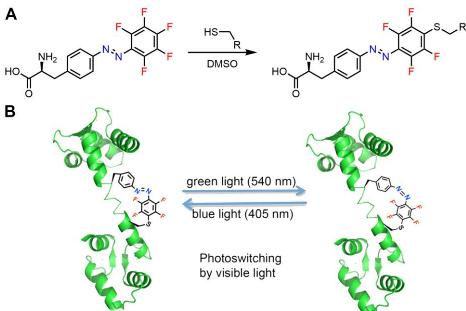
Scheme 4.4: Reaction of 4-(pentafluorophenyl)azo-L-phenylalanine with free thiols via nucleophilic aromatic substitution (A), and the application of this amino acid in the photomodulation of Calmodulin (B). Images adapted from Hoppmann et al. , 2015. 33
