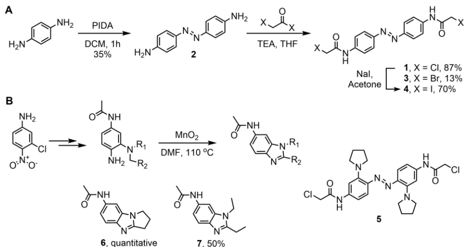
Scheme 4.3: Synthesis of azobenzene crosslinkers 1 , 3 and 4 , (A) and the attempted synthesis of crosslinker 5 showing efficient conversion of ortho-aminoalkanes to benzimidazoles (B).
