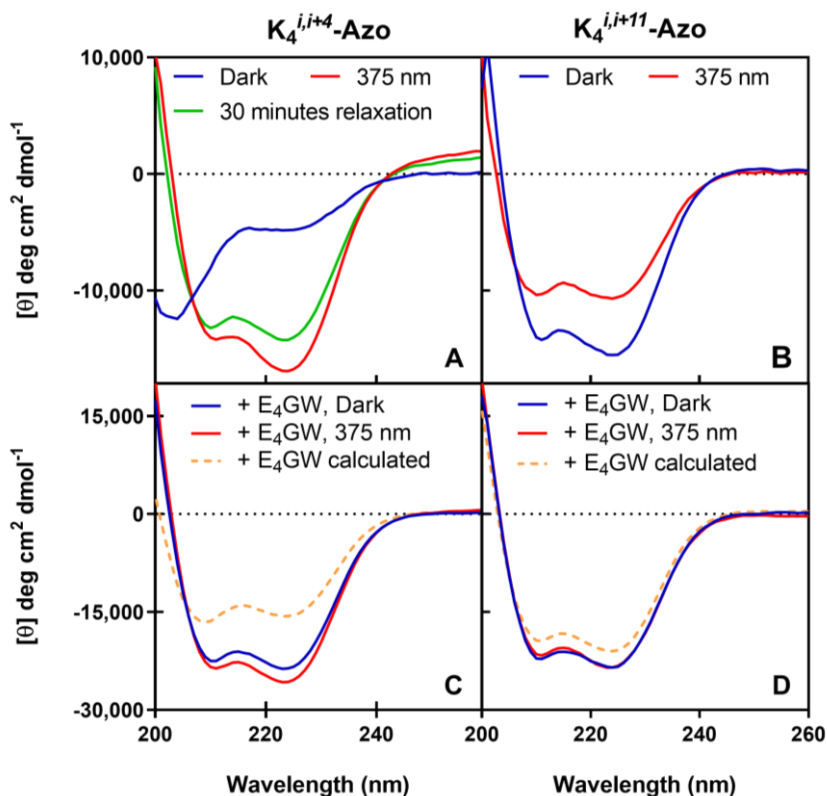
Figure 4.2: CD spectra of K_4 peptide variants crosslinked with azobenzenes. CD measurements are shown for peptide K_4^{i,i+4} -Azo (A) and peptide K_4^{i,i+11} -Azo (B) and their respective complexes with peptide E_4 GW (C and D). Spectra are measured at 25 \mu M peptide concentration in PBS at pH 7.4, with samples either kept in the dark before measurements, or illuminated for 3 minutes with 375 nm light. Calculated coiled-coil spectra are for the less folded azobenzene isomer ( Trans isomer for K_4^{i,i+4} -Azo, C; Cis isomer for K_4^{i,i+11} -Azo, D).
