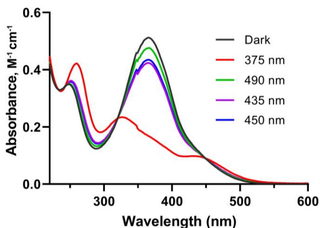
Figure S4.1: UV-Vis spectra at different photostationary states of peptide K_{3,i,i+4} -Azo showing successful switching between cis -, (375 nm) and trans -dominant (490 nm) photostationary states. Spectra were measured at 50 \mu M peptide concentration in PBS buffer, pH 7.4.
