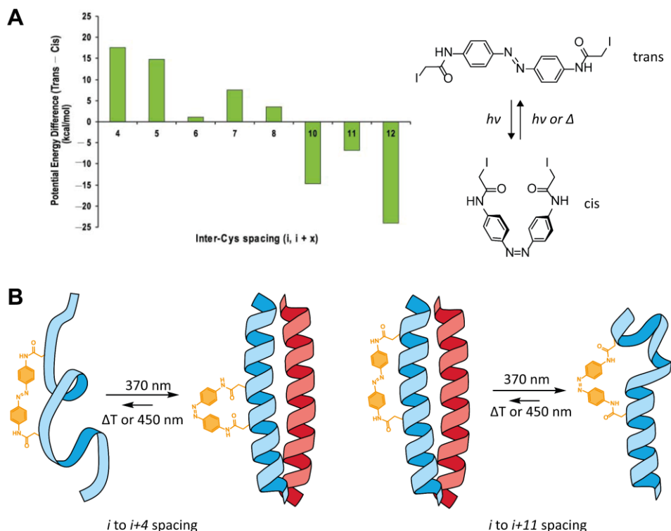
Scheme 4.1: Azobenzene based crosslinker for the photocontrol of peptide structure and the effect of crosslinker spacing on the difference in calculated peptide folding energy when switching between cis and trans isomers (A). Images adapted from Flint et. al. 14 Schematic representation of incorporating photoactive crosslinkers in a heterodimeric coiled-coil system (B). Depending on spacing between the attachment points of the crosslinker, either the light or the dark state can be expected to show the highest coiled-coil characteristics.
